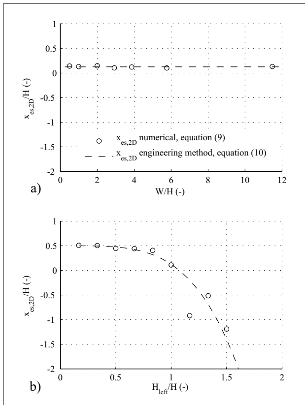
Figure 3. Values of the equivalent source position x_{es,2D} for attenuation term A'_{s,2D} , a) as a function of the canyon width W with H = 19.2 m, b) as a function of the left building height H_{left} with W = 19.2 m.
