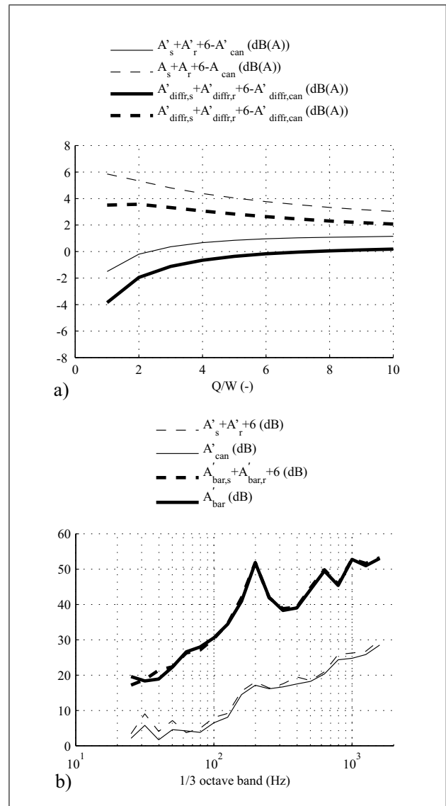
Figure 10. a) Broadband error of splitting the attenuation term A'_{can} into A'_s + A'_r , and A'_{can} into A_s + A_r . Results have been averaged over all receiver positions, b) Results at Q = 10W averaged over all receiver positions.
