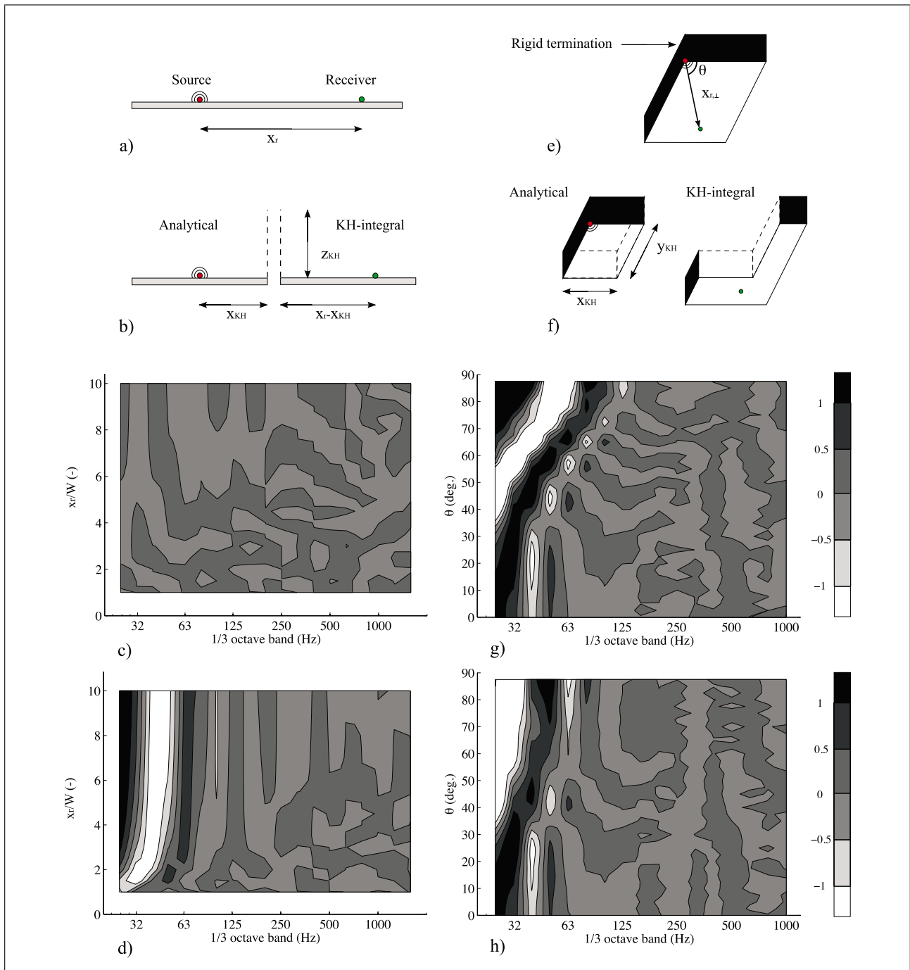
Figure A2. a) 2D configuration studied, b) Two-stage computational approach with analytical results at x_{KH} and KH-integral approach from x_{KH} = W/2 + 2 m to receiver at x_r . c) Error of the KH-integral approach for z_{KH} = 30 m for W = 19.2 m, d) Error of the KH-integral approach for z_{KH} = 30 m for W = 19.2 / \cos(\theta) m and \theta = 80 deg., e) 3D configuration studied, f) Two-stage computational approach with analytical results at x_{KH} = W/2 + 2 m and KH-integral approach to receiver at x_{r,\perp} = 20W , W = 19.2 m, g) Error of the KH-integral approach for z_{KH} = 30 m for y_{KH} = 4W according to configurations (c,d) of Figure 2. h) Error of the KH-integral approach for z_{KH} = 30 m for y_{KH} = 3W/2 + 2 m according to configurations (e,f) of Figure 2 with T = 3W/2 . Errors in dB.
