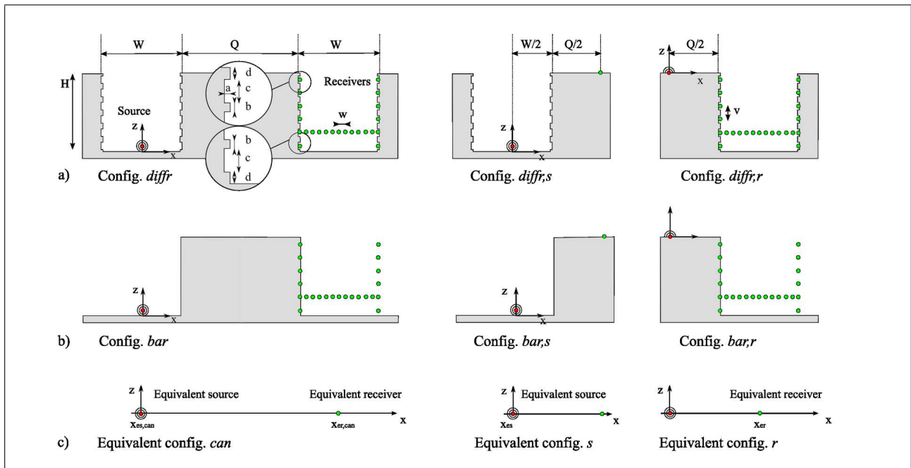
Figure 1. Configurations studied with numerical parameters a = 0.16 m, b = 1.28 m, c = 1.92 m, d = 0.64 m, v = c + b = 3.2 m, w = 1.6 m, z_s = 0.5 m when the source is located in the street and z_s = H when the source is located at roof level, W = 19.2 m, H = 19.2 m, Q is variable. (a) Configurations for which the shielding attenuation terms A_{diff} , A_{diff,s} and A_{diff,r} apply, (b) Configurations for which the barrier attenuation terms A_{bar} , A_{bar,s} and A_{bar,r} apply, (c) Equivalent configurations for which the shielding attenuation terms A_{can} , A_s and A_r apply.
