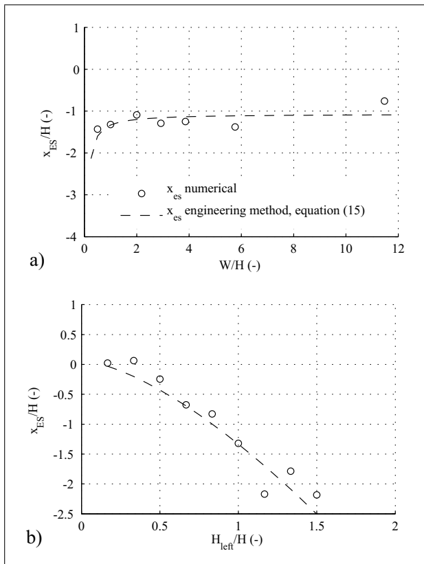
Figure 7. Values of the equivalent source position x_{es} for 3D attenuation term A'_s for configuration (a) of Figure 2 and y_r=0 m, as a function of the canyon width W with H = 19.2 m, b) as a function of the left building height H_{left} with W = 19.2 m.
