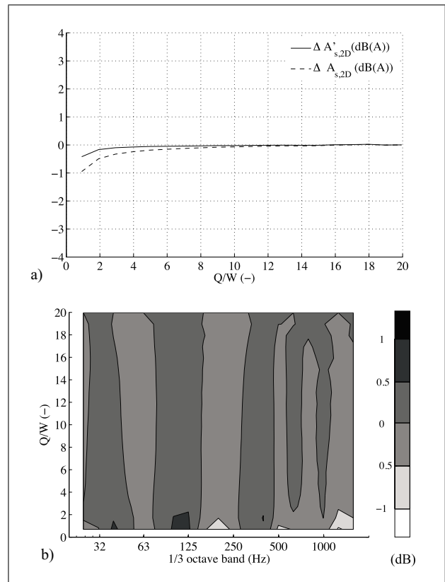
Figure 4. Attenuation terms computed from configurations diff,r,s and bar,r,s of Figure 1, a) \Delta A_{s,2D} and \Delta A'_{s,2D} in dB(A), b) \Delta A'_{s,2D} .
