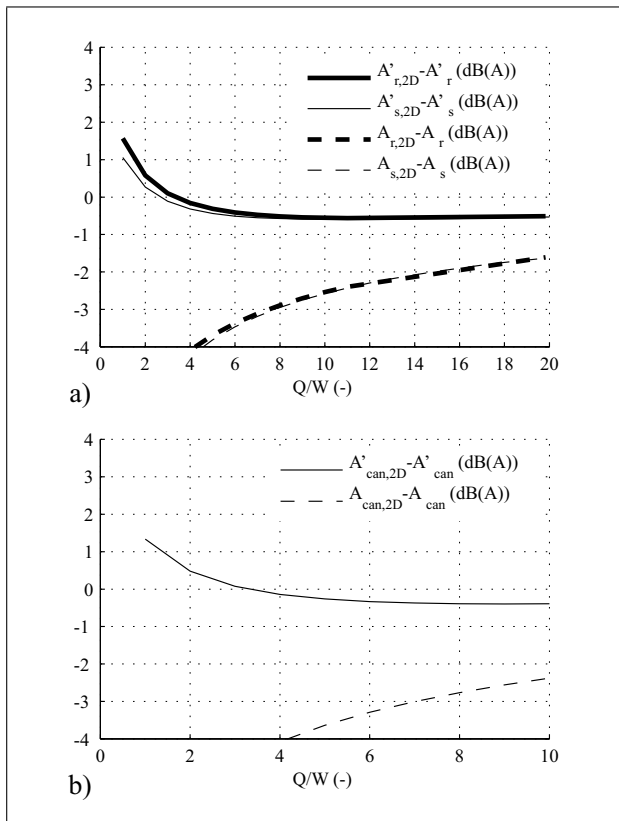
Figure 11. Broadband difference between 2D and 3D attenuation terms. Results have been averaged over all receiver positions, a) separate source and receiver environment terms, b) total canyon term.
