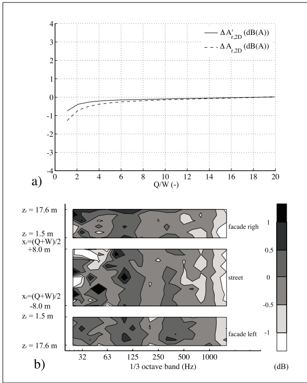
Figure 5. Attenuation terms computed from configurations diff,r and bar,r of Figure 1, a) \Delta A'_{r,2D} and \Delta A_{r,2D} , averaged over all receiver positions, b) \Delta A'_{r,2D} ( Q = 2W ) as a function of the receiver position and third octave bands.
