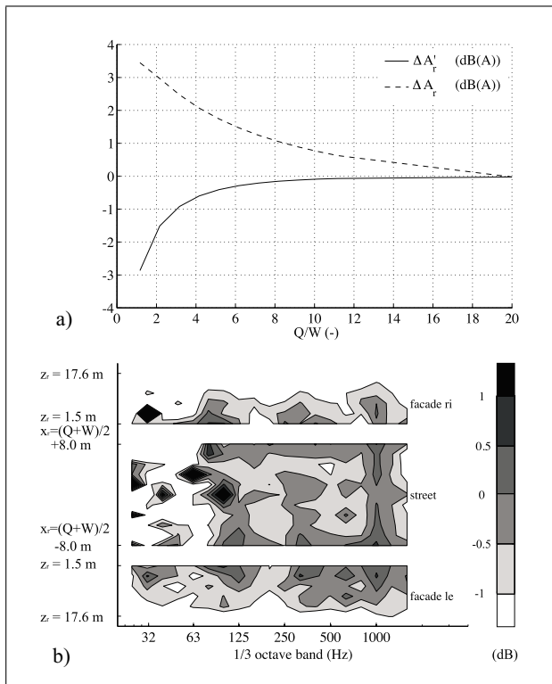
Figure 9. Attenuation terms computed from configurations diff,r and bar,r of Figure 1, a) \Delta A'_r and \Delta A_r , averaged over all receiver positions, b) \Delta A'_r(Q = 4W) as a function of the receiver position and third octave bands.
