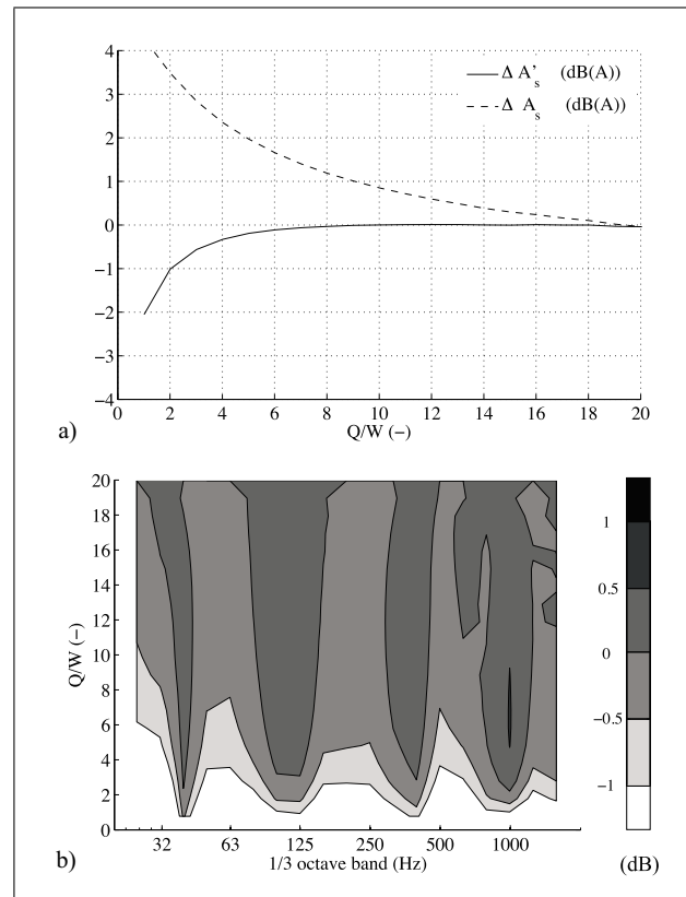
Figure 8. Attenuation terms computed from configurations diff,r,s and bar,s of Figure 1, a) \Delta A_s and \Delta A'_s in dB(A), b) \Delta A'_s .
