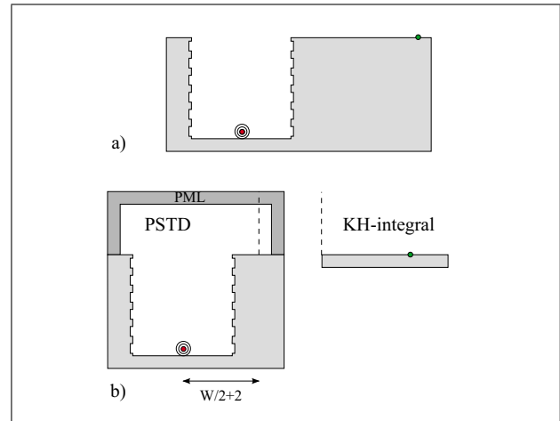
Figure A1. Two-step numerical approach to solve configuration of a), b) Application of PSTD method to solve source region part, and evaluation of the KH-integral equation to solve the region over roof level height.
