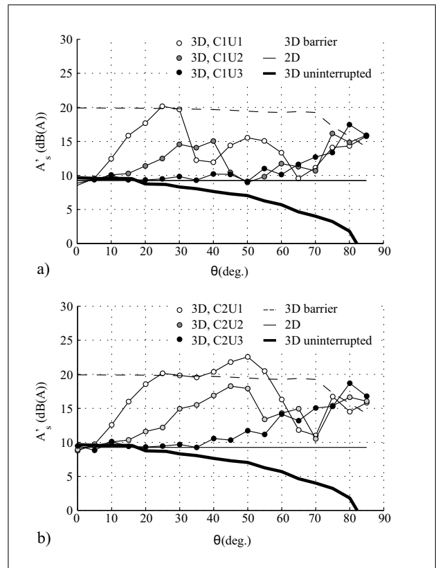
Figure 13. Broadband values up to 1 kHz at Q = 40W for configurations (a) and (c) as depicted in Figure 2.
