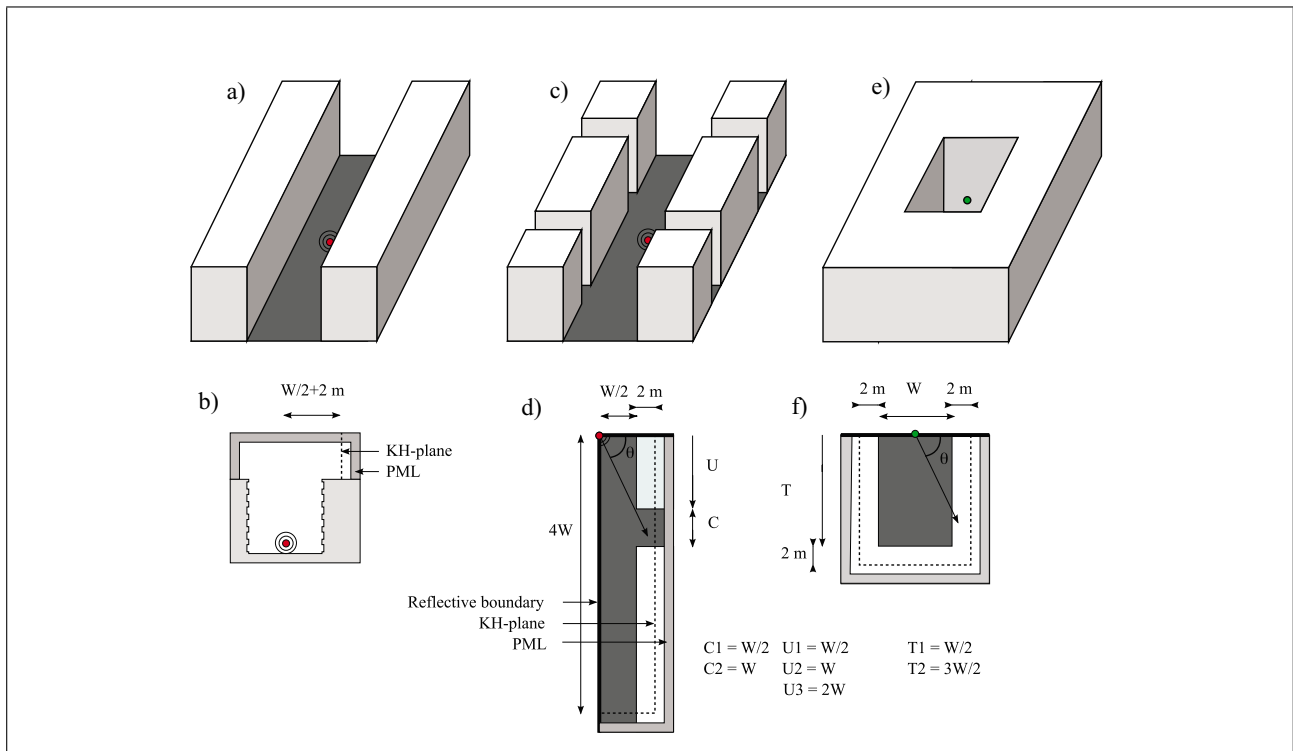
Figure 2. 3D configurations studied, a) Graphical representation infinite street, b) Computational approach shown by cross section at y = 0 . A 2.5 D transform is applied to the 2D results. c) Graphical representation of finite street with cross streets, d) Computational approach of c), shown by top view, e) Graphical representation of courtyard, f) Computational approach of e), shown by top view.
