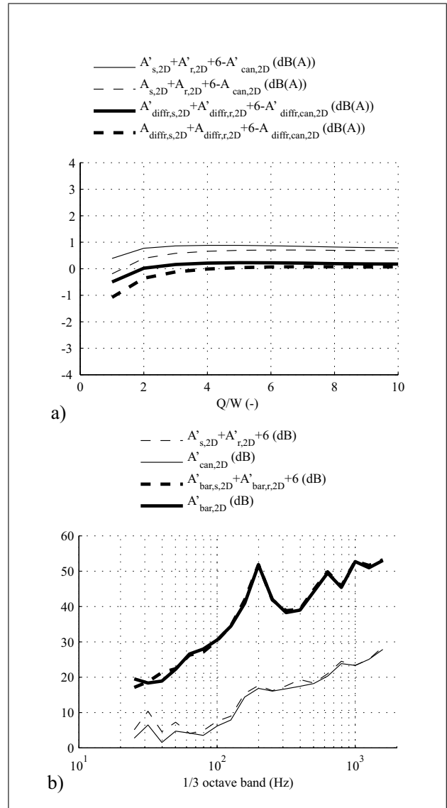
Figure 6. a) Broadband error of splitting the attenuation term A'_{can,2D} into A'_{s,2D} + A'_{r,2D} , and A_{can,2D} into A_{s,2D} + A_{r,2D} . Results have been averaged over all receiver positions, b) Results at Q = 10W averaged over all receiver positions.
