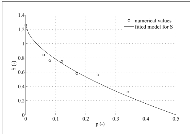
Figure 14. Angular averaged values of S = (A'_{\text{bar},s}(\theta = 0^\circ) - \bar{A}'_s) / (A'_{\text{bar},s}(\theta = 0^\circ) - A'_{s,2D}) for the various interrupted street configurations and the infinite street, p is the angular fraction of façades openings in the horizontal plane as seen from the source.
