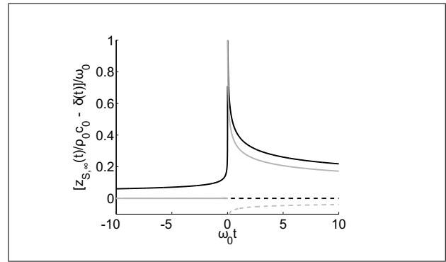
Figure 2. Continuous part of the normalized impulse response [z_{S,\infty}(t)/\rho_0 c_0 - \delta(t)]/\omega_0 as a function of the normalized time \omega_0 t : (solid line) real and (dashed line) imaginary parts of the first extension (in black) in equation (48) and second extension (in grey) in equation (52) of the Delany and Bazley impedance model of a semi-infinite ground.
