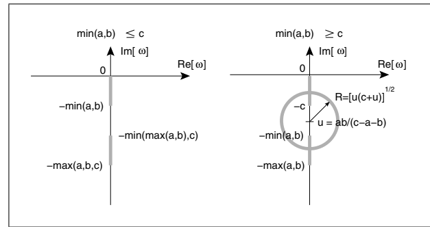
Figure 1. Branch cuts in the \omega -plane of the function [(a - i\omega)(b - i\omega)/(-i\omega(c - i\omega))]^{1/2} , where a , b and c are all real positive coefficients.
