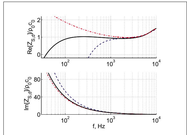
Figure 3. Real and imaginary parts of a rigidly backed layer of thickness d = 0.01 \text{ m} and of air flow resistivity \sigma_0 = 100 \text{ kPa s m}^{-2} as a function of the frequency f : (dashed line) Delany and Bazley model, (solid line) Miki model and (dash-dotted line) modified Miki model.
