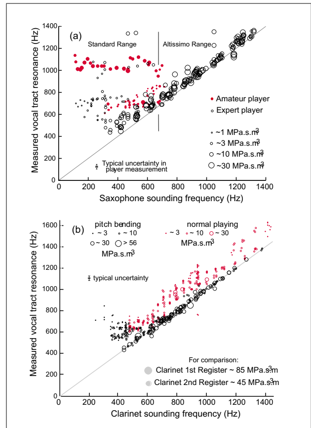
Figure 8. The relationship between the measured resonance frequency f_{\text{res}} of the vocal tract and the sounding frequency f_0 , i.e. the fundamental of the note played, for the clarinet and tenor saxophone. In each figure the continuous line indicates the relationship f_{\text{res}} = f_0 . In Figure 8a, the open and filled circles indicate expert and amateur players respectively. In Figure 8b the open and filled circles indicate measurements during normal playing and pitch bending respectively. In each figure the size of the symbol indicates the magnitude of the impedance peak. After [65] and [53] respectively.
