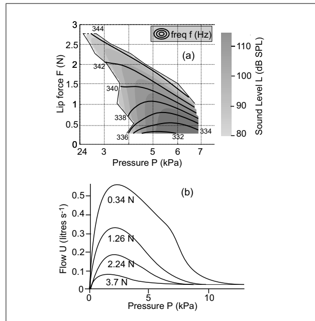
Figure 4. Two of the control parameters available to clarinetists are the pressure in the mouth and the force with which the lip presses the reed. Both are varied using a playing machine in the upper plot [17]. Dark lines show contours of equal frequency (values shown in Hz) and the grey scale shows the sound level measured near the bell. Illustrative sound samples from this plot are available online [38]. These results can be interpreted in terms of the lower plot, showing the flow U past the reed as a function of the pressure difference across the reed (after Dalmont and Frappé [37]). The different curves are for different forces applied by the ‘lip’ to the reed.
