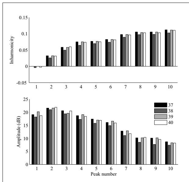
Figure 6. At the top, inharmonicity (with the fundamental frequency f_0 = 142.4 Hz of saxophones 37 and 39 taken as reference) and at the bottom, amplitudes of the maxima of the 10 first input impedance peaks for the Bb3 fingering (all the holes closed) on the four saxophones.
