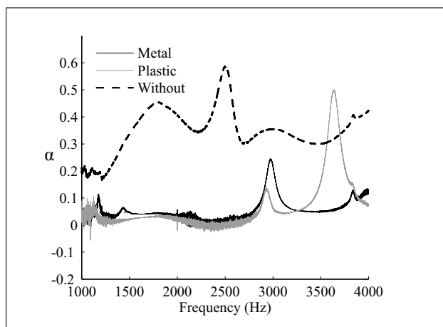
Figure 3. Absorption coefficient of the pads as a function of frequency. Pad with metal resonator (black), with plastic resonator (grey) and without a resonator (black dashed).
