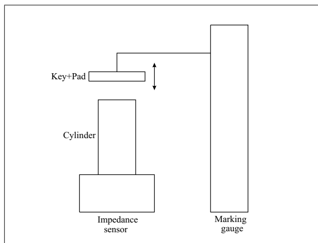
Figure 2. Technical sketch of the experimental protocol used for the measurements of the cylinder input impedance.
