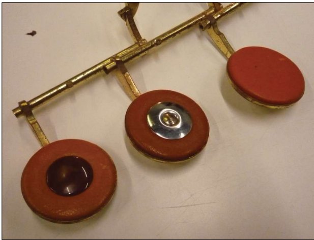
Figure 1. Three kinds of pads: with a plastic resonator on the left, with a metal resonator in the middle, and without a resonator on the right. (Color online)
