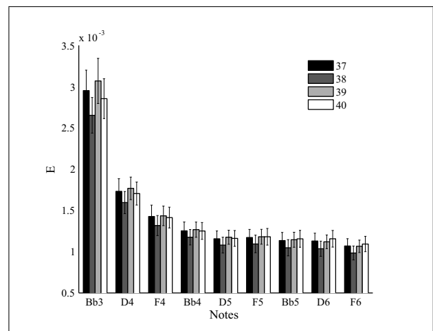
Figure 16. The mean and its standard error of the efficiency for each note and each saxophone. The mean is calculated on 30 samples (10 musicians * 3 repetitions).
