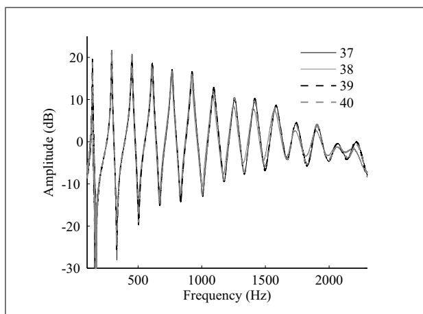
Figure 5. Comparison of the input impedance amplitude of the four saxophones for the fingering of B \flat 3 (all toneholes closed). 37 and 39 are the saxophones with plastic resonators (black continuous and dashed lines), 38 is the one without resonators (grey continuous line) and 40 the one with metal resonators (grey dashed line).
