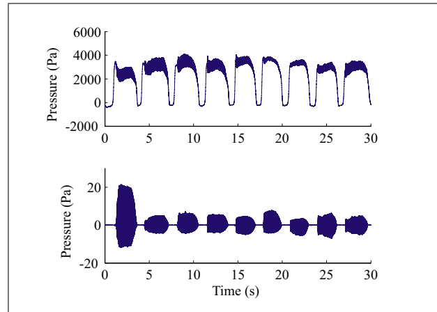
Figure 13. Example of the pressures recorded while the musician is playing the arpeggio: mouth pressure (top) and pressure at the bell (bottom).
