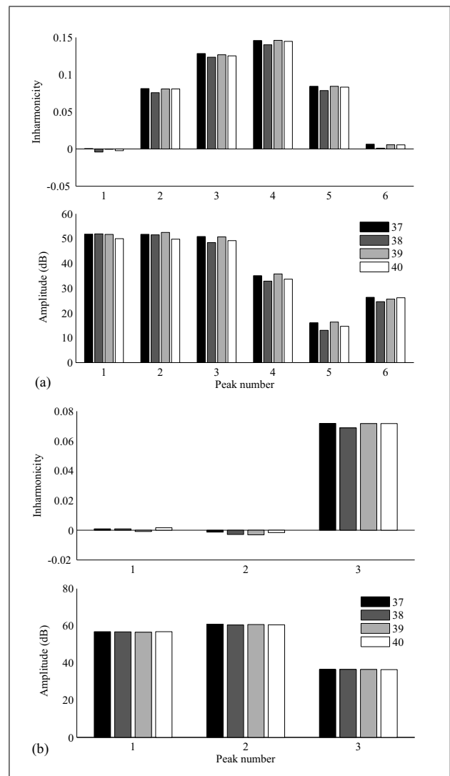
Figure 7. (a) At the top, inharmonicity (with the average fundamental frequency f_0 = 218.1 Hz of saxophones 37 and 39 taken as reference) and at the bottom, amplitudes of the maxima of the 6 first input impedance peaks for the F4 fingering (about half of the holes closed) on the four saxophones. (b) At the top, inharmonicity (with the average fundamental frequency f_0 = 548.5 Hz of saxophones 37 and 39 taken as reference) and at the bottom, amplitudes of the maxima of the 3 first input impedance peaks for the F6 fingering (all but one keys raised) on the four saxophones.
