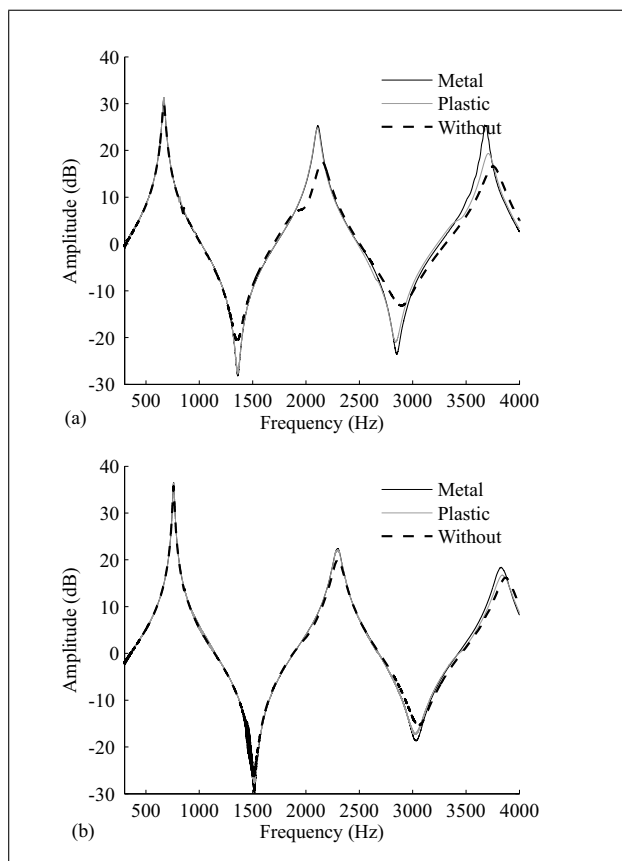
Figure 4. Input impedance (dimensionless) of the pipe terminated by the three pads (pad with metal resonator in black, with plastic resonator in grey and without a resonator in black dashed line) at a height of (a) 1 mm and (b) 5 mm.
