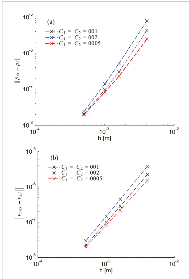
Figure 3. Convergence of the approximation using linear P1/P1 elements (a) pressure field (b) velocity in the x-direction.
