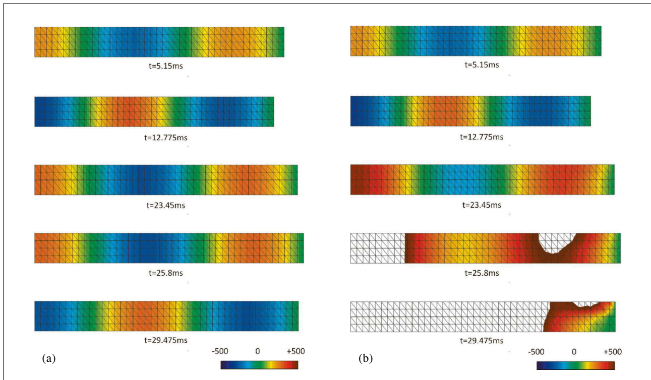
Figure 2. Snapshots of the acoustic pressure in Pa inside the 2D duct at different time steps considering (a) all stabilization terms and (b) removing the ALE stabilization terms.
