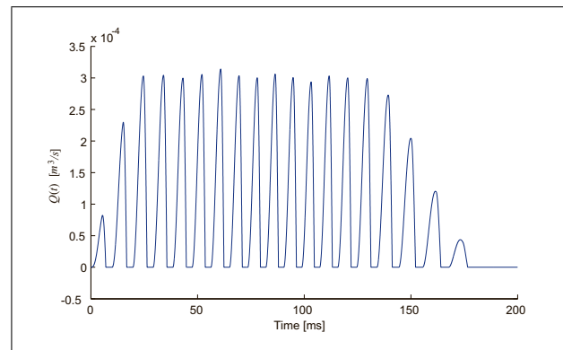
Figure 5. Train of glottal pulses introduced at the glottis to generate the diphthong /ai/.
