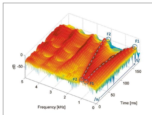
Figure 8. Spectrogram of the acoustic pressure at the node located close to mouth exit from Figure 7. Formant trajectories from /a/ to /i/ have been highlighted.
