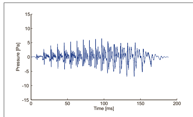
Figure 7. Time evolution of the acoustic pressure at a point close to the mouth exit. When converted to audio, it produces the sound /ai/.
