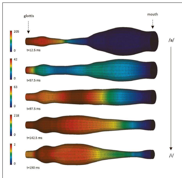
Figure 6. Snapshots at five different time instants showing the transition from vowel /a/ to /i/. The acoustic pressure in Pa at the boundaries of the vocal tract and its shape evolution can be appreciated.
