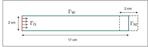
Figure 1. Sketch of the two dimensional duct example used to test the stabilized FEM approach for the ALE mixed wave equation. \Gamma_G stands for the boundary where the input signal \mathbf{u}_g(t) is introduced, \Gamma_W the duct walls and \Gamma_M the duct exit, which moves sinusoidally backward and forward.
