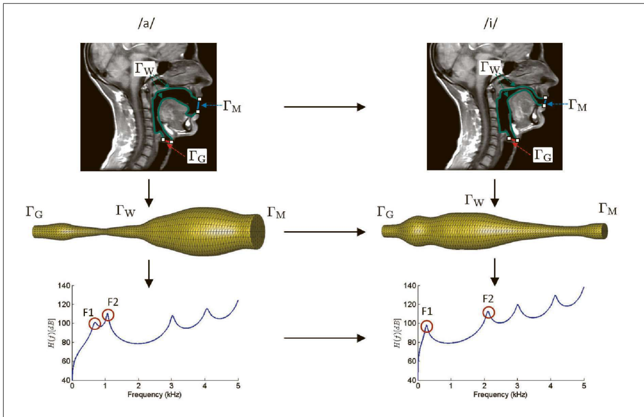
Figure 4. Sketch for the numerical production of vowels. From magnetic resonance imaging (MRI), data is obtained for the computation of vocal tract transfer functions (VTTF). The left column corresponds to vowel /a/ and the right column to vowel /i/. The diphthong /ai/ involves transiting from /a/ to /i/.
