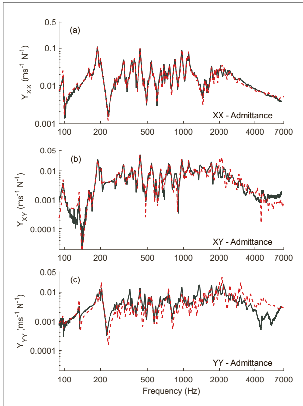
Figure 4. Measured admittances in the plane perpendicular to the string axis (green solid curve, colour online) and the fitted admittances to them (red dashed curve, colour online) for (a) XX admittance (b) XY admittance and (c) YY admittance. Note that the vertical scales are different in (a) and (b)-(c).
