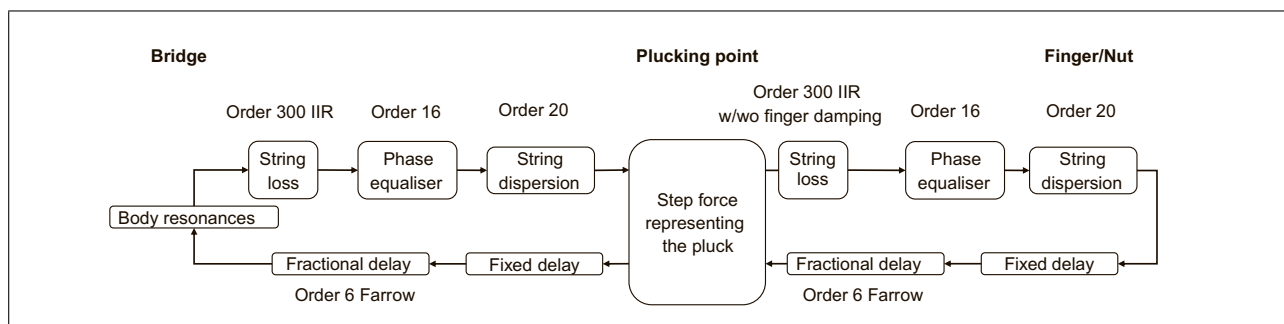
Figure 5. Schematic of the plucked-string model.
