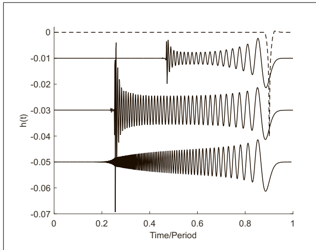
Figure 3. Equivalent reflection function (impulse response of the loop filter) designed for the finger side of a damped cello C_2 string, perfectly flexible (dashed line) and stiff (top solid line). The natural frequency of the string is 65.4 Hz, \beta = 0.1 , frequency-dependent Q factor based on the data in Table I, bending stiffness is 6.2 \times 10^{-4} \text{ Nm}^2 , sampling frequency 6 \times 10^4 \text{ Hz} . The middle solid line is the same as the top solid line except the Q factor of the string modes is assumed constant at 600, and the number of poles in the dispersion filter is increased from 20 to 40. The bottom solid line is the equivalent of the middle solid line but damping is modelled using the constant-Q reflection function of Equation (5), and dispersion is implemented based on the method proposed in [8]. Note the spike-like behaviour in the top solid line at non-dimensionalised time 0.47, and more vividly, in the middle solid line at non-dimensionalised time 0.25, resulting from frequencies above the design frequency of the dispersion filter.
