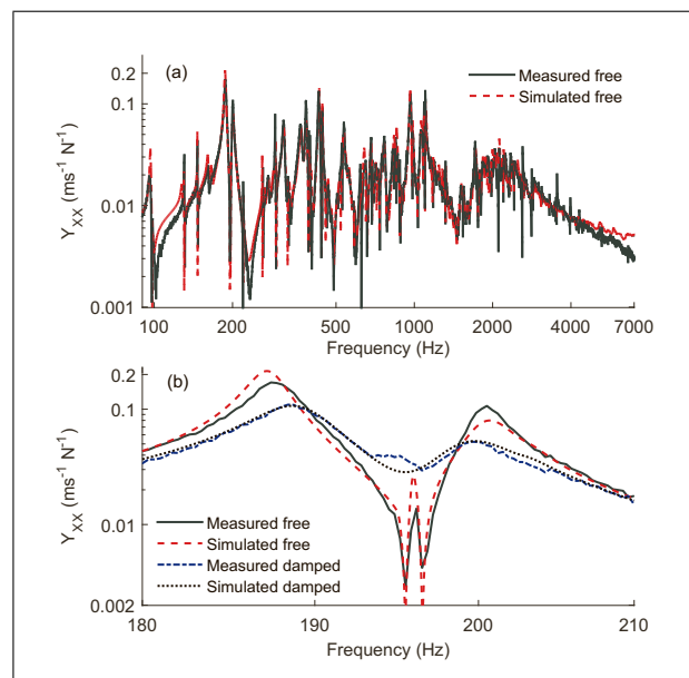
Figure 9. Simulated versus measured bridge admittance in the X direction when all four strings are free to vibrate (a), and a zoomed version of that plot covering only the “wolf-note” area (b). Both measured and simulated data for the strings-damped case are also included in the lower plot for comparison.
