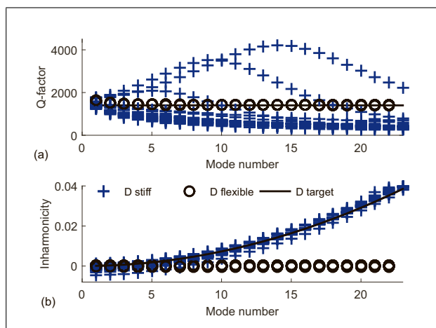
Figure 10. Trend of Q factor (a) and inharmonicity (i.e. [(f_n/nf_0)^2 - 1] ) (b) versus the string mode number for stiff and flexible open D_3 cello string, based on the old implementation. The strings had rigid terminations and the results were extracted from 10 seconds of simulated plucked response. \beta was varied in 20 steps and the results are overlaid.
