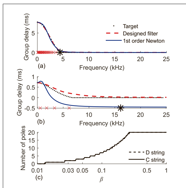
Figure 2. Group delay of the designed filter (dashed line) for the finger side (a), and the bridge side (b) of the open cello C 2 string compared to the desired response (dotted line), and a filter designed with first-order Newton's approximation (solid line). The crosses show the position of the poles used in the designed filter and the star shows the upper limit of the design frequency range. A constant group delay is assigned for the frequencies beyond that range. (c) shows the order of the dispersion filter for the C 2 and D 3 strings as a function of \beta .
