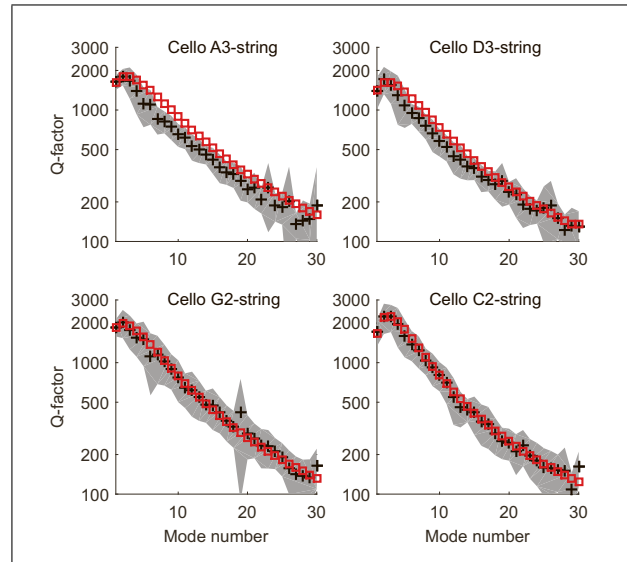
Figure 1. Average measured Q factor (plus signs) plus/minus one standard deviation (grey shade) for D’Addario Kaplan Solutions cello strings. The red squares show the fit of Equation (6) to the measured data.
