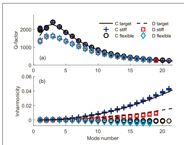
Figure 6. Trend of the Q factor (a) and inharmonicity (i.e. [(f_n/nf_0)^2 - 1] ) (b) versus the string mode number for the stiff and flexible open C_2 and D_3 cello strings. All strings were terminated at rigid boundaries and the results are extracted from 10 s of simulated plucked response. \beta is varied in 20 steps and the results are overlaid.
