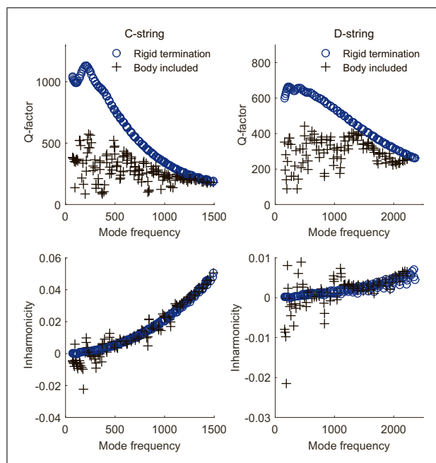
Figure 7. Trend of Q factor (upper plots) and inharmonicity (lower plots) versus the string mode frequencies for the stiff C_2 (left plots) and the stiff D_3 (right plots) cello strings. Circles show the case when the strings are terminated at rigid boundaries and plus signs show the case when the flexible body is included in the simulations. The first 11 semitones have been “played” on each string and the results were extracted from 10 seconds of a simulated plucked response.
