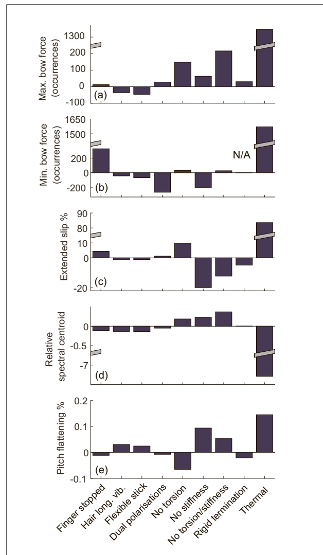
Figure 4. The variation of (a) maximum bow force; (b) minimum bow force; (c) increase in the slip-to-stick ratio as a percentage of its theoretical value; (d) spectral centroid relative to the fundamental frequency; and (e) pitch flattening as a percentage of the fundamental frequency, relative to their values for the base case. Different cases shown on the horizontal axis are defined in the text. Note the broken vertical scales in cases (a)–(d).
