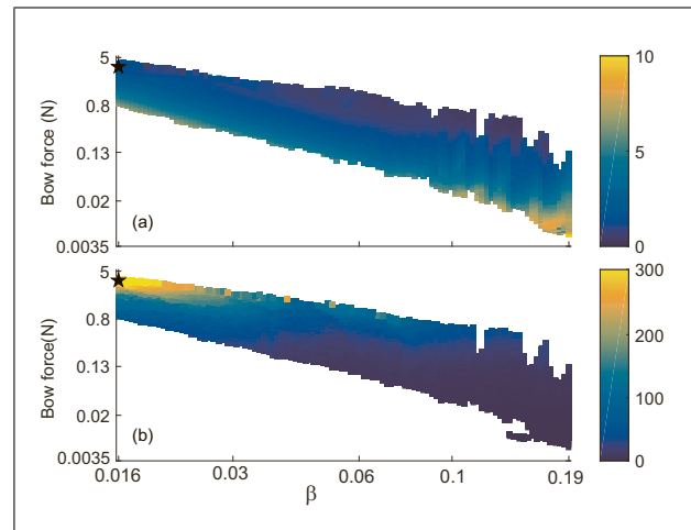
Figure 7. Region of the Schelleng diagram exhibiting Helmholtz motion, with colour scales indicating the amplitude of fluctuations as a percentage of the nominal values for (a) the bow force (unit \times 100 N/N) and (b) the bow speed (unit \times 100 (m/s)/(m/s)), based on the data from the “Dual-polarisations” and “Hair long. vib.” cases of an open D_3 string. The stars indicate the instances plotted in Figure 8.
