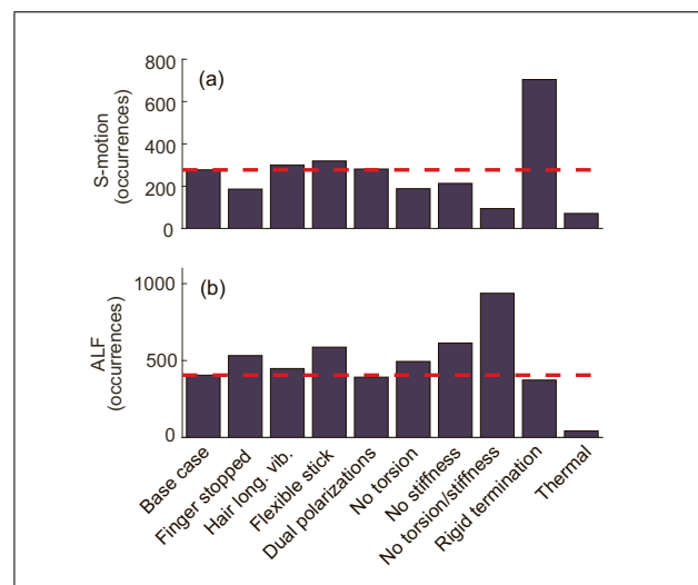
Figure 6. Comparing the total number of S-motion (a) and ALF note (b) occurrences for different cases defined in the text.
