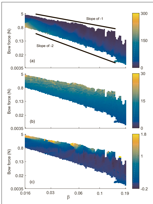
Figure 3. Different metrics of waveforms for the base case, in the \beta - F_N plane. (a) The increase in the slip-to-stick ratio as a percentage of its theoretical value (unit \times 100 s/s), (b) the spectral centroid relative to the fundamental frequency (unit Hz/Hz), and (c) the pitch flattening as a percentage of the fundamental frequency (unit \times 100 Hz/Hz). The theoretical slopes for the minimum and maximum bow force are shown in (a) by thick diagonal lines to guide the eye.
