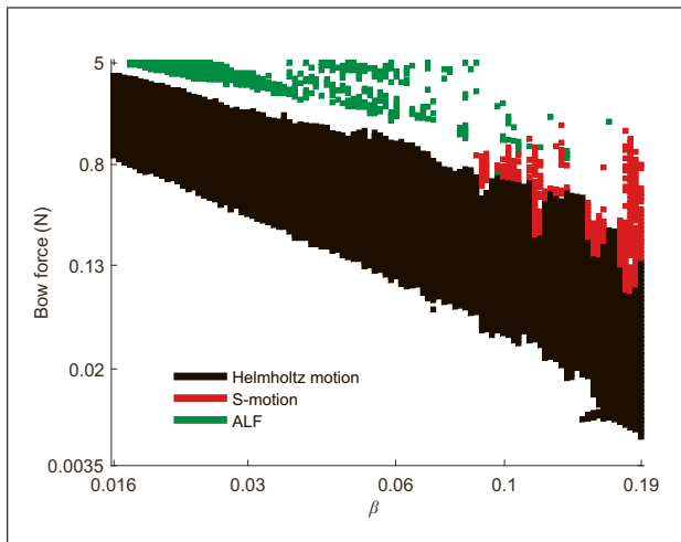
Figure 2. Schelleng diagram calculated for the base case.
