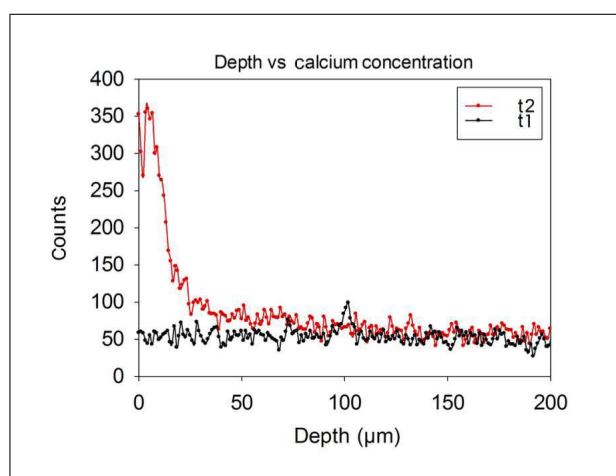
Figure 5. Penetration depth ( \mu\text{m} ) of Calcium: the concentration measured through semi-quantitative analysis (EDX) along the red line (colour online) of Figure 4a decreases to its minimum around 30\mu\text{m} of depth.
