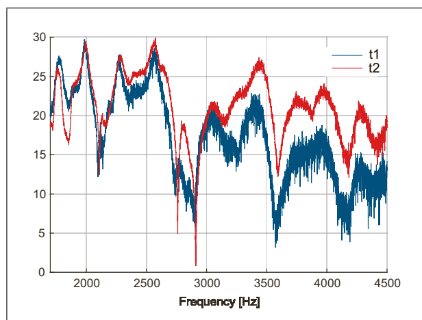
Figure 8. FRF (from 1700 to 4300 Hz) measured on a soundboard before and after the application of the ground-coat.
