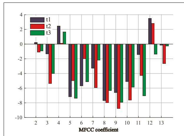
Figure 12. MFCC values.
