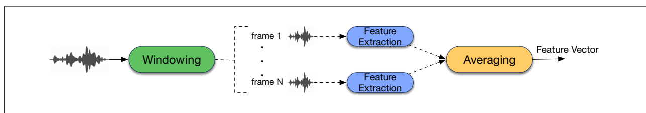
Figure 9. Overall scheme of the feature extraction procedure.
