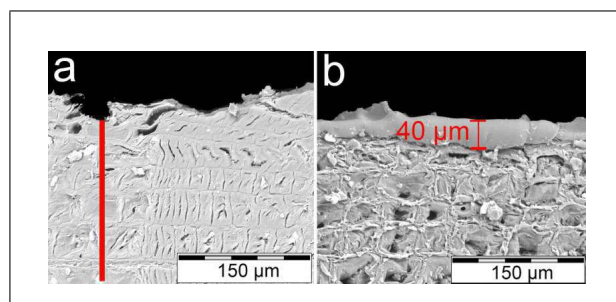
Figure 4. Electronic microscopy BSE image (1000X) of the cross section after applying ground coat (t2): the red line represents the semi-quantitative analysis (EDX) trajectory performed transversely through the section (a); electronic microscopy BSE image (1000X) of the cross section after applying ground coat and varnish (t3): thickness measure of varnish stratum (b).
