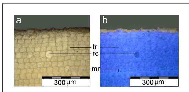
Figure 3. Optical microscopy images (20X) of the cross section after applying ground coat and varnish (t3): visible light (a) and UV induced fluorescence (b). Anatomical wooden structures: medullary ray (mr), resin canal (rc), tracheid and/or fiber tracheid (tr).
