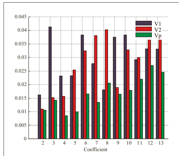
Figure 11. Variation of the MFCC coefficients in three cases: from t1 to t2 (V1), from t2 to t3 (V2) and during the execution of different musicians with a reference instrument (Vp).
