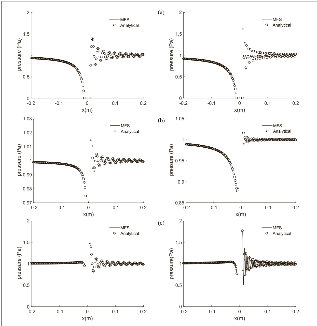
Figure 4. Pressure along a line of receivers for the case of the fluid-filled sphere, calculated using the MFS and analytically. Left column corresponds to a frequency of 38 kHz and right column to a frequency of 120 kHz. The properties of the filling fluid are: (a) fish-flesh; (b) air; (c) quasi-rigid sphere.
