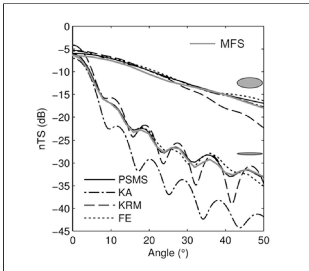
Figure 5. Comparison of MFS method scattering results with results from PSMS, KA, KRM and FEM models from [30]. Results plot length-normalized target strength (nTS) for two prolate spheroids with ka = 12 and kb = 5 (upper lines) and ka = 13 and kb = 1 (lower lines) as a function of angle off broadside. Curves for PSMS, KA, KRM and FEM from Figure 4 of [10].
