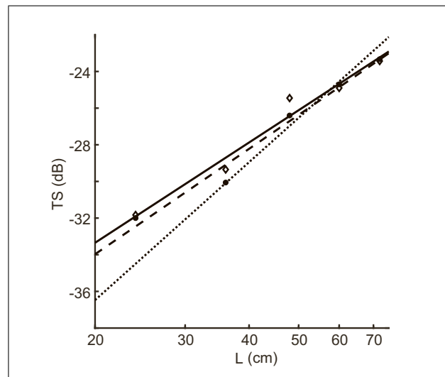
Figure 12. Regression curves for TS_{\max} versus fish length considering ventral fish aspect calculated at 70 kHz (dashed line) and 120 kHz (continuous line) at d = 18 m corresponding to Equations (13) and (14), respectively. Calculated values are included as circles (70 kHz) and diamonds (120 kHz). Regression fit of mean TS -to-fish length from experimental results ventrally measured at 120 kHz in [3] are included (dotted line).
