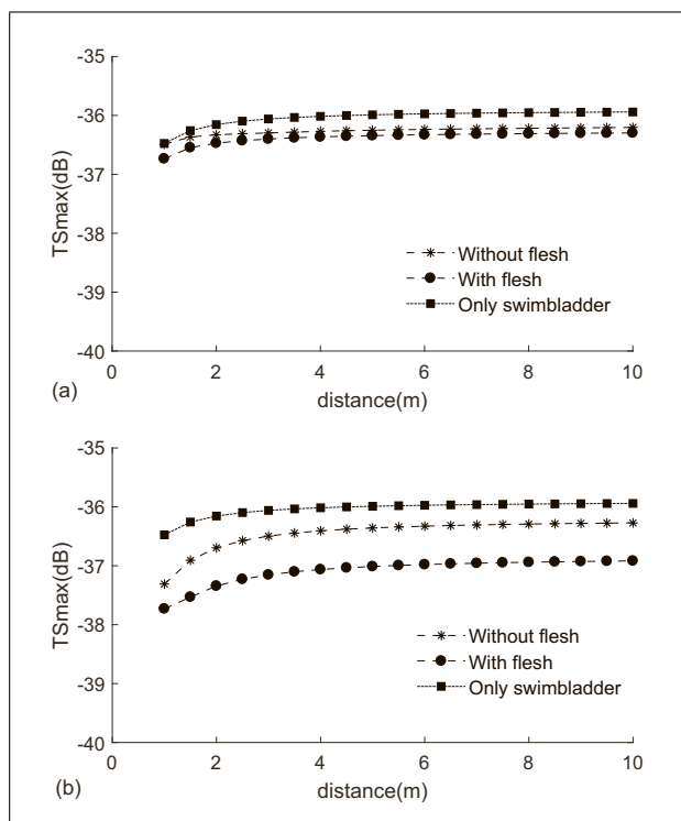
Figure 8. Calculated TS at 70 kHz for ventral (a) and dorsal (b) insonification for a 18 cm fish as a function of the distance between the transducer and the fish. Three curves are represented, corresponding to the calculation considering the complete fish model including the flesh (dashed line with circle marks), just considering the spine and swim bladder (dashed line with star marks), and only accounting for the swim bladder (dotted line with square marks).
