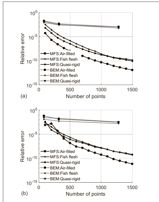
Figure 3. Relative error of the numerical calculations for the benchmark fluid-filled sphere problem, considering increasing numbers of collocation points (or elements, in the case of the BEM), for: a) 38 kHz; b) 120 kHz.
