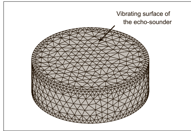
Figure 2. Discretization of the echo-sounder's surface in small triangles.
