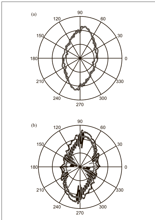
Figure 10. Dorsal ( 90^\circ ) and ventral ( 270^\circ ) TS directivity on the x - y plane calculated at 70 kHz (dashed) and 120 kHz (continuous line) for fish length L = 24 cm (a) and L = 72 cm (b). Transducer-to-fish distance d = 6 m (black line) and d = 18 m (grey line).
