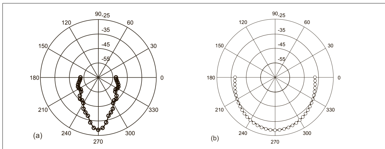
Figure 7. Directivity plot calculated 10 m away from the spheroids, considering the MFS (full line) and the BEM (circles): a) prolate spheroid with transverse radius of 1.24 cm; b) prolate spheroid with transverse radius of 6.18 cm.
