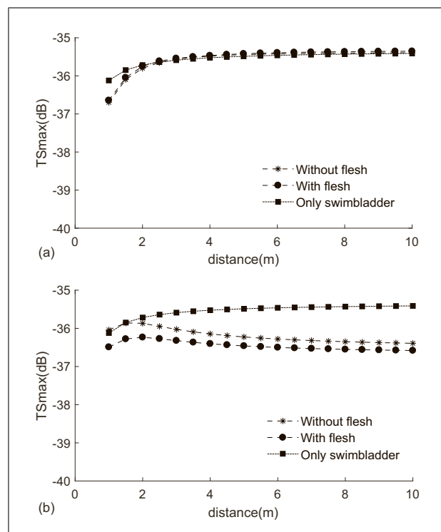
Figure 9. Calculated TS at 120 kHz for ventral (a) and dorsal (b) insonification for a 18 cm fish as a function of the distance between the transducer and the fish. Three curves are represented, corresponding to the calculation considering the complete fish model including the flesh (dashed line with circle marks), just considering the spine and swim bladder (dashed line with star marks), and only accounting for the swim bladder (dotted line with square marks).
