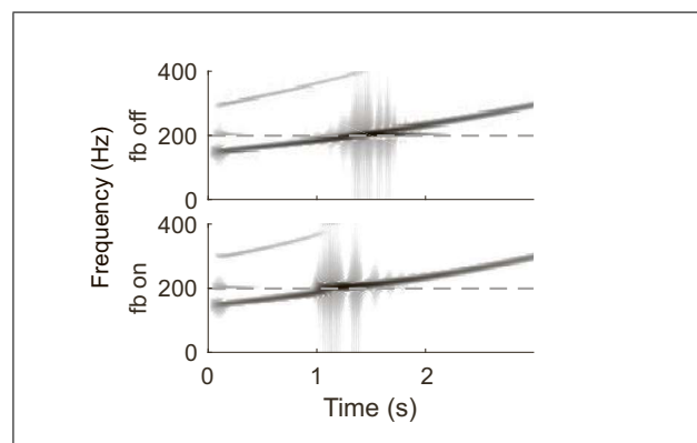
Figure 6. Spectrogram of pressure at lips during glide for [i]. Top: without feedback ( Q_{pc} = 0 ). Bottom: with feedback ( Q_{pc} = 0.1 ). Dashed gray line is f_{R1} .
