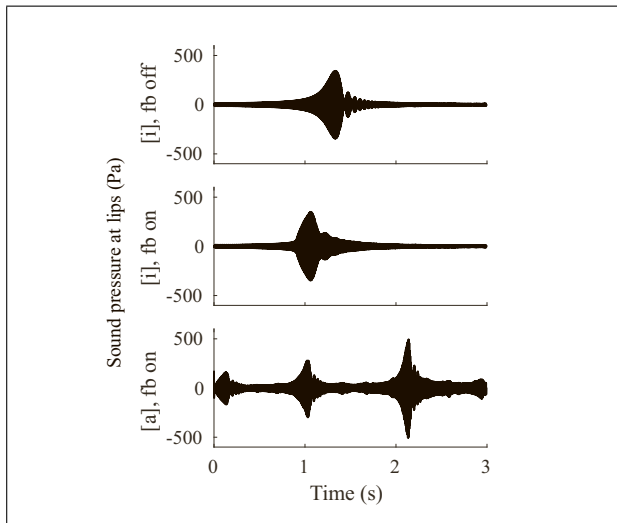
Figure 8. Sound pressures at the lips during upward glides. Top: [i] without feedback ( Q_{pc} = 0 ). Middle: [i] with feedback ( Q_{pc} = 0.1 ). Bottom: [a] with feedback ( Q_{pc} = 0.1 ).
