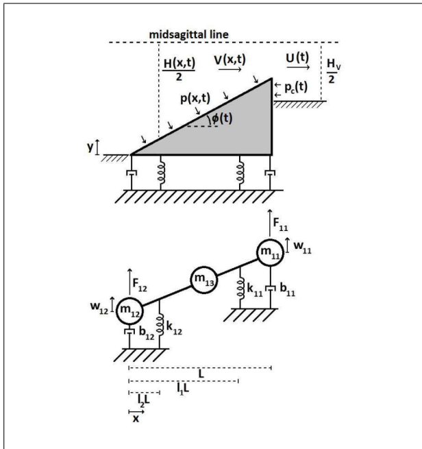
Figure 1. Top: The geometry of the glottis model with the trachea to the left and the vocal tract to the right. Bottom: Lumped-element representation of the lower vocal fold ( j = 1 ) with two degrees of freedom.
