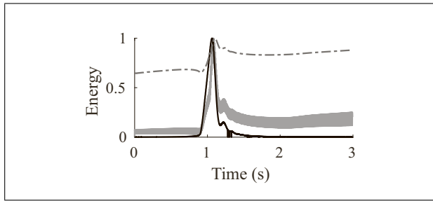
Figure 9. Normalised envelope of energy in VT acoustics (solid black) and in the glottal flow U (dashed gray), and energy in vocal fold vibrations (solid gray) in upward glide for [i] with Q_{pc} = 0.1 .
