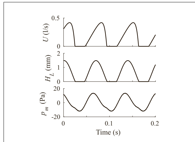
Figure 4. Simulated pulse shapes for [i] with feedback ( Q_{pc} = 0.1 ) before the glide begins: glottal flow U , glottal gap H_L , and sound pressure at the lips p_m .
