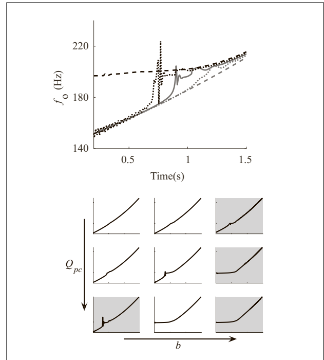
Figure 11. Top: f_o trajectories for [i] with different values of Q_{pc} : gray dashed 0.0, gray dotted 0.05, gray solid 0.1, black dotted 0.15, and black dashed 0.2. Bottom: f_o trajectories for [i] qualitatively as Q_{pc} and \beta increase in the direction of the arrow. Light gray background indicates that small parameter changes can lead to loss of quasi-stable glides.
