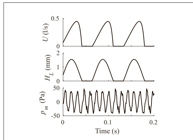
Figure 5. Simulated pulse shapes for [α] with feedback ( Q_{pc} = 0.1 ) before glide: glottal flow U , glottal gap H_L , and sound pressure at the lips p_m .
