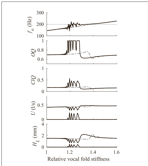
Figure 10. Upward (dashed gray) and downward (solid black) glides for vowel [i] with Q_{pc} = 0.04 . Shown are fundamental frequency f_o ( f_{R1} indicated by horizontal gray line), open quotient OQ , closing quotient ClQ , and the envelopes of glottal flow U and gap H_L . On the x-axis, relative vocal fold stiffness refers to the coefficient of the K^0 matrix in equations (18) and (19).
