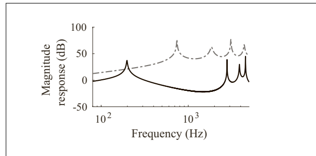
Figure 3. The magnitude responses of the VT acoustic loads obtained by simulating output for an impulse input for [a] (dashed gray) and [i] (solid black). The response of [a] has been raised by 50 dB for clarity.
