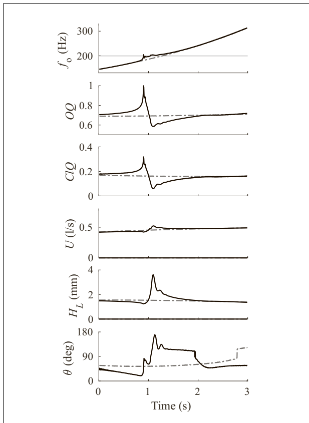
Figure 7. Glide for [i] with feedback ( Q_{pc} = 0.1 ) (solid black) and without feedback ( Q_{pc} = 0 ) (dashed gray). Shown are fundamental frequency f_o (horizontal gray line is f_{R1} ), open quotient OQ , closing quotient CIQ , envelopes of glottal flow U and gap H_L , and phase difference \theta between m_{j1} and m_{j2} .
