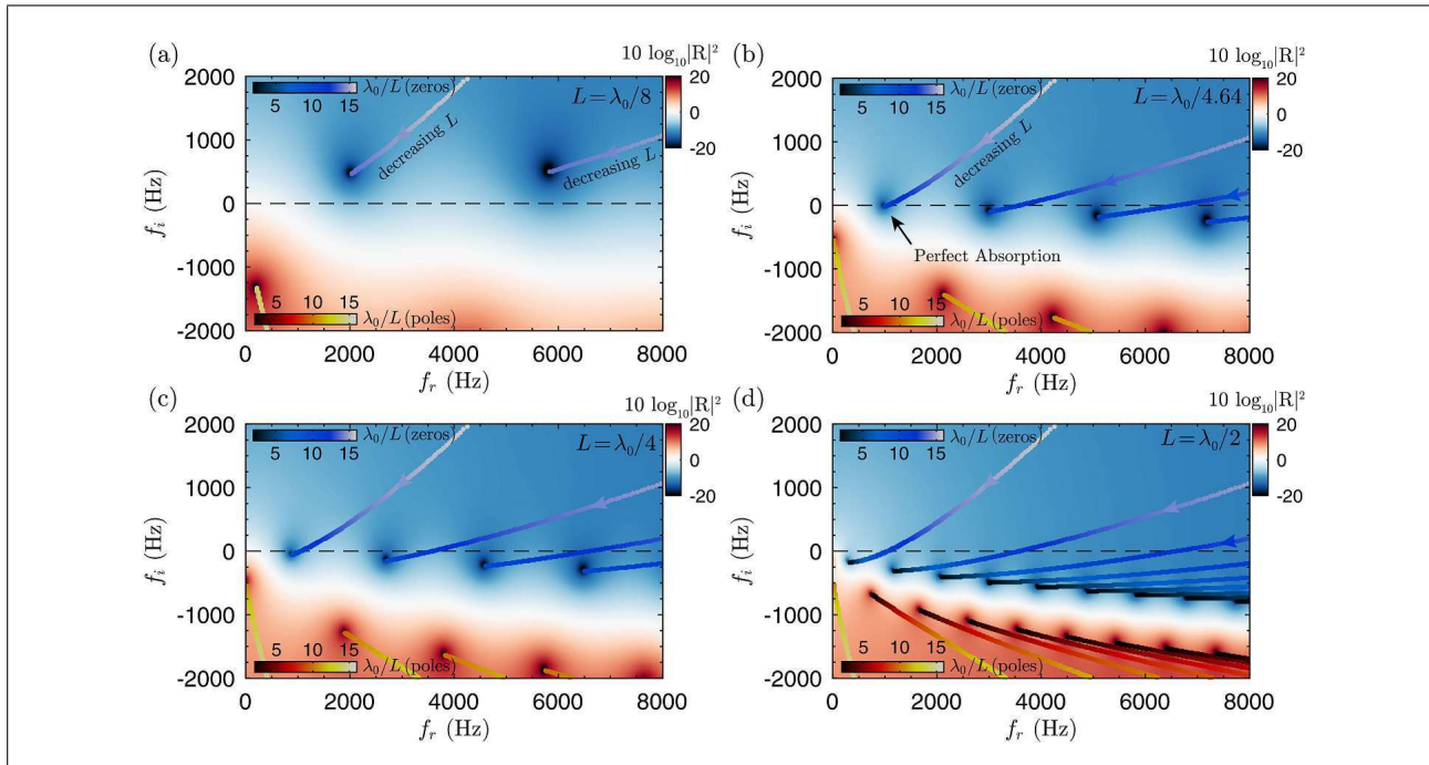
Figure 3. (Colour online) Complex frequency representation of the reflection coefficient in logarithmic scale. The trajectories of the zeros (blueish) and poles (reddish) lines are marked as a function of the panel thickness. (a) L = \lambda_0/8 , (b) Critically coupled configuration, L = \lambda_0/4.64 , (c) L = \lambda_0/4 and (d) L = \lambda_0/2 .
