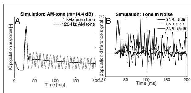
Figure 1. A : Simulated IC population responses to a 4-kHz pure tone and a 120-Hz, 4-kHz AM tone of 70 dB SPL. The detection cue is the rms of the difference signal of the waveforms. B : Difference signal between simulated responses for noise and TiN epochs of a 70dB-SPL 4-kHz pure tones embedded in a one-octave wide white noise for different SNRs. The rms of the difference signal is the simulated detection cue.
