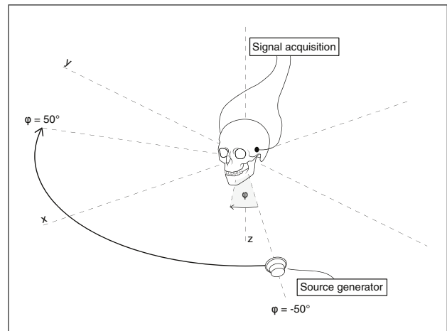
Figure 1. Sketch of the experimental setup in the horizontal plane: A loudspeaker is connected to a source generator (PC) and emits a chirp signal at each angle \varphi ranging from -50^\circ to 50^\circ along a half circle at various distances to the skull. The resulting vibration of the skull is recorded through two passive sensors glued to the hypothetical ear locations. They are connected to the signal acquisition system, consisting of a sound card connected to a PC.
