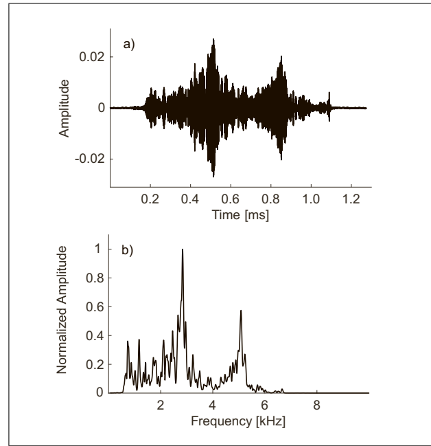
Figure 2. a) Exemplary waveform of a recorded signal at one of the sensors. b) Frequency spectrum of the same signal.
