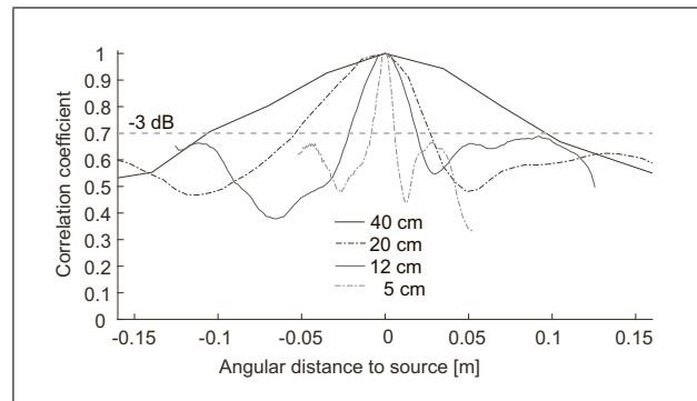
Figure 3. Normalized focusing functions along the curvilinear abscissa for sources in front of the center of the skull ( \varphi = 0^\circ ) and at different distances to the skull. The distance of the measurement points to the skull decreases from 40 cm, down to 20 cm, 12 cm and 5 cm (different curves). There is a clear trend of increasing resolution (decreasing -3 dB width of the curves) with decreasing distance.
