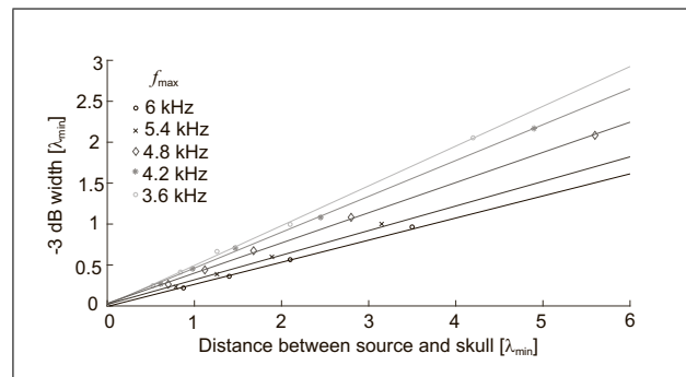
Figure 4. -3 dB width values of the focusing functions for sources at different distances to the skull (x-axis) and maximum frequencies f_{max} of the signal. The slope of each linear fit, which corresponds to the apparent aperture A in Equation 4, is approximately 10 cm for all curves.
