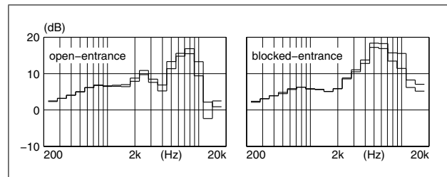
Figure 17. Measurements with 3-mm microphone displacement between (both microphone and blockage are displaced). Brüel and Kjør 4128, HRTF at approximately 90° azimuth measured with probe microphone.
