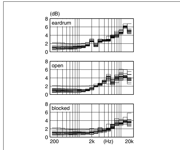
Figure 6. \sigma(L_{FA}) for 14 headphones (thin lines, mean in heavy line), when literature data are used for \Delta L (equation 5) and measurements carried out at eardrum (top), open entrance (middle) and blocked entrance (bottom).
