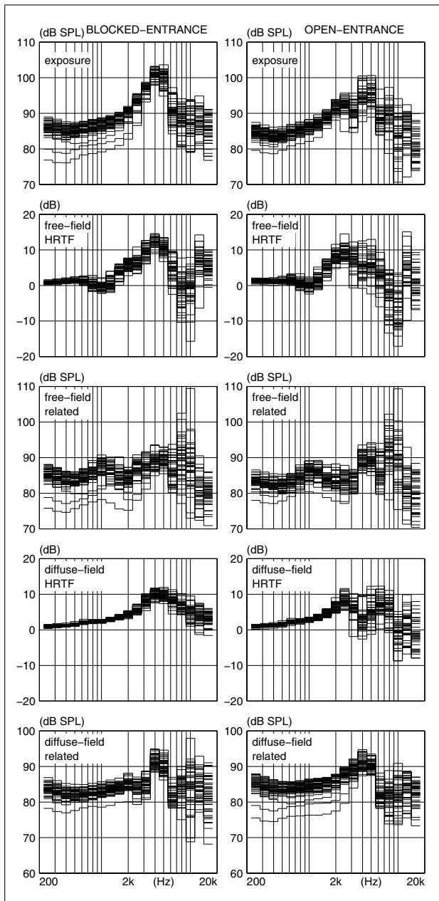
Figure 4. Blocked- and open-entrance data for 40 individuals (thin lines, means in heavy lines). Top panels show exposure data for the Sony MDR 102 headphone, 2nd row shows the free-field HRTFs, 3rd row shows the resulting free-field related levels, 4th row shows the diffuse-field HRTFs, and bottom row shows the diffuse-field related levels. A-weighting and summation give free-field related A-weighted levels of 98.5 dB (blocked-entrance mean) and 98.3 dB (open-entrance mean), and diffuse-field related A-weighted levels of 98.5 (blocked-entrance mean) and 97.6 dB (open-entrance mean).
