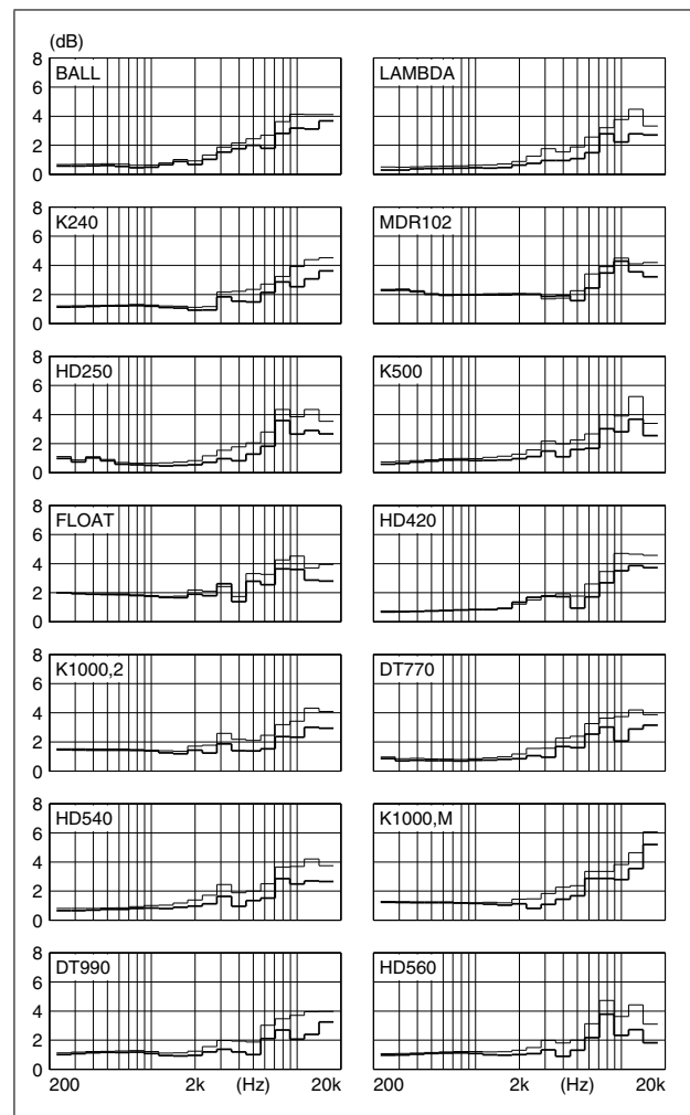
Figure 16. \sigma(L_{DF}) for 14 headphones. Derived from complete calculation of L_{BE} - \Delta L_{BE} (heavy line) or from the combined variances of L_{BE} and \Delta L_{BE} (thin line) (respectively left and right side of equation (11)).
