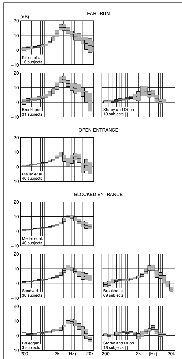
Figure 8. Diffuse-field HRTFs from literature, mean (heavy line) and mean \pm one standard deviation (grey area). Eardrum data from Killion et al. [39, 40], Bronkhorst [15], and Storey and Dillon [18], open entrance data from Møller et al. [7, 8], and blocked entrance data from Møller et al. [7, 8], Sandvad [11], Bronkhorst [15], and Brügger [17], Storey and Dillon [18].
