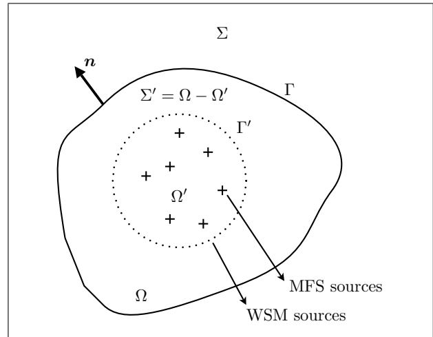
Figure 1. Vibrating body and the virtual sources.
