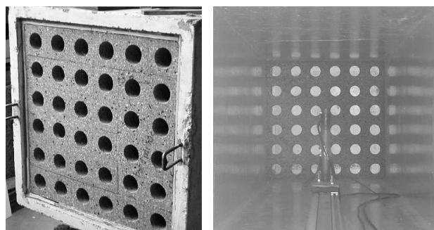
Figure 10. 90 mm thick double porosity (u160) sample in the Big Kundt Tube. Left: exterior view, right: interior view.
