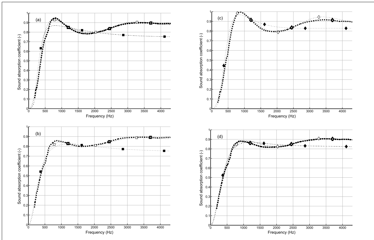
Figure 17. Small Kundt Tube, 45 mm thick layer, validation for configurations A and B. (a) Configuration A, double porosity: comparison between experimental data (thick black square) and analytical model in case of F_d = 1 (thin black square) and F_d = F_d(\omega) (thin black filled square). (b) Configuration A, heterogeneous material: comparison between experimental data (thick black square) and analytical model in case of F_d = 1 (thin black square) and F_d = F_d(\omega) (thin black filled square). (c) Configuration B, double porosity: comparison between experimental data (thick black diamond) and analytical model in case of F_d = 1 (thin black diamond) and F_d = F_d(\omega) (thin black filled diamond). (d) Configuration B, heterogeneous material: comparison between experimental data (thick black diamond) and analytical model in case of F_d = 1 (thin black diamond) and F_d = F_d(\omega) (thin black filled diamond).
