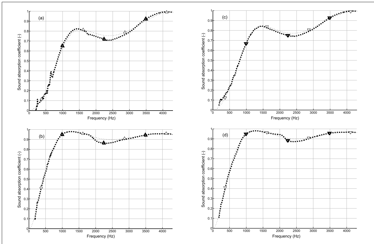
Figure 18. Small Kundt Tube, 45 mm thick layer, validation for configurations C and D. (a) Configuration C, double porosity: comparison between experimental data (thick black triangle) and analytical model in case of F_d = F_d(\omega) (thin black triangle). (b) Configuration C, heterogeneous material: comparison between experimental data (inverted thick black triangle) and analytical model in case of F_d = F_d(\omega) (inverted thin black triangle). (c) Configuration D, double porosity: comparison between experimental data (inverted thick black triangle) and analytical model in case of F_d = F_d(\omega) (inverted thin black triangle). (d) Configuration D, heterogeneous material: comparison between experimental data (inverted thick black triangle) and analytical model in case of F_d = F_d(\omega) (inverted thin black triangle).
