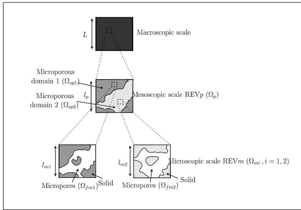
Figure 1. The three scales of the considered heterogeneous medium.
