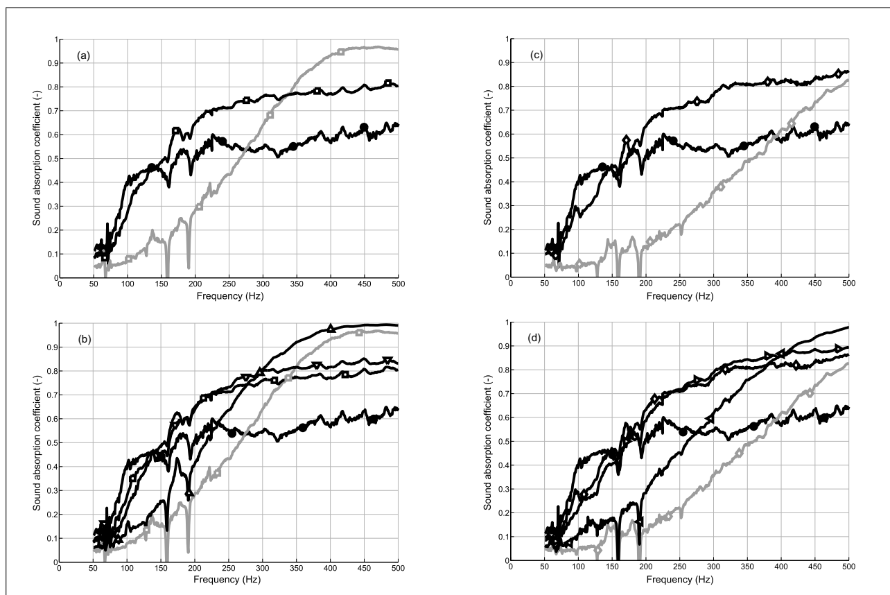
Figure 15. Big Kundt Tube, rockwool as frame microporous material, 90 mm thick layer: influence of the inclusions. (a) Configuration with 6 x 6 perforations, cases of double porosity (grey square) and rockwool-melamine heterogeneous material (black square) compared to the homogeneous rockwool (black circle). (b) As in (a), with two hybrid solutions: a 45 mm thick double porosity layer in the front and a 45 mm thick rockwool-melamine heterogeneous layer in the back (black triangle) and the vice versa (inverted black triangle). (c) Configuration with 7 x 7 perforations, cases of double porosity (grey diamond) and rockwool-melamine heterogeneous material (black circle) compared to the homogeneous rockwool (black circle). (d) As in (c), with two hybrid solutions: a 45 mm thick double porosity layer in the front and a 45 mm thick rockwool-melamine heterogeneous layer in the back (black triangle \leftarrow ) and the vice versa (inverted black triangle \rightarrow ).
