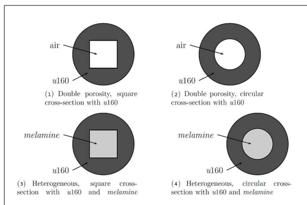
Figure 7. Sketch of cross-section geometries for a sample in the SKT or in the MKT, representing a single cell.
