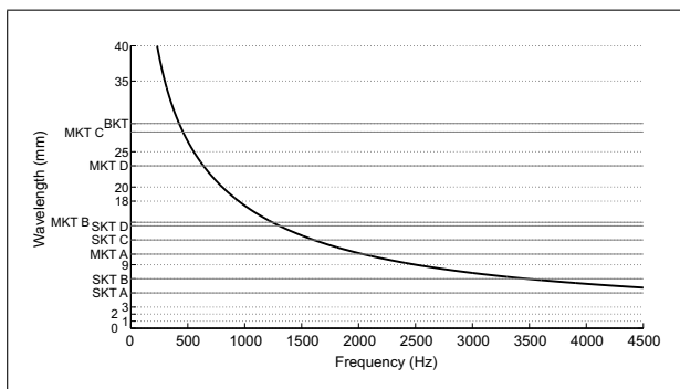
Figure 19. Wavelength in the u160 (rigid frame model) compared with the size of mesoheterogeneities: SKT refers to Small Kundt Tube, MKT to Medium and BKT to Big; A-B-C-D represent the configurations described in Tables II and III.
