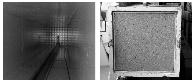
Figure 6. Big Kundt Tube. Left: rail and microphone in the interior, right: preparation of a sample of u160.
