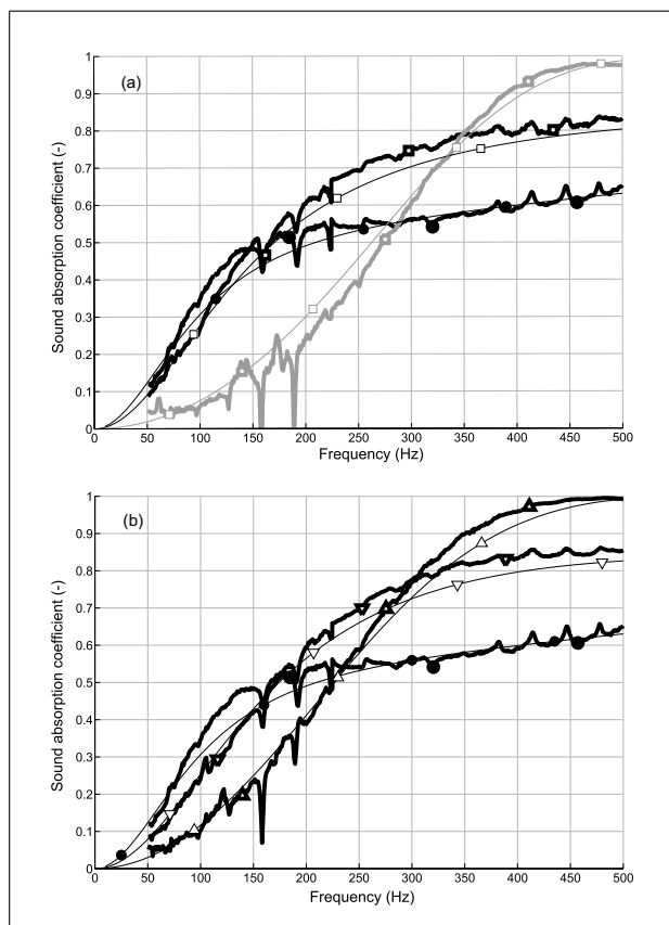
Figure 16. Big Kundt Tube, 90 mm thick layer composed of u160 and melamine, validation. (a) Comparison between experimental (solid line) and analytical (thin line) data: single porosity u160 (black circle), double porosity u160 (grey square), heterogeneous u160-melamine (black square). (b) Comparison between experimental (solid line) and analytical (thin line) data: single porosity u160 (black circle), hybrid configuration with double porosity u160 in front and heterogeneous u160-melamine on the back (black triangle), hybrid configuration in vice versa (inverted black triangle).
