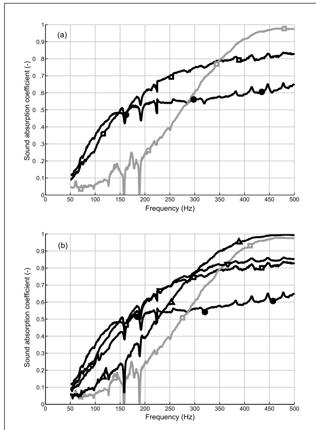
Figure 13. Big Kundt Tube, 90 mm thick layer, influence of the inclusions. (a) Cases of double porosity (grey square) and u160-melamine heterogeneous material (black square), compared to the homogeneous u160 (black circle). (b) As in (a), with two hybrid solutions: a 45 mm thick double porosity layer in the front and a 45 mm thick u160-melamine heterogeneous layer in the back (black triangle) and the vice versa (inverted black triangle).
