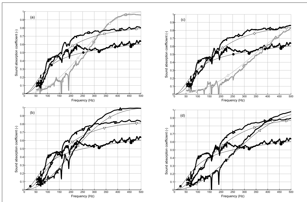
Figure 22. Big Kundt Tube, 90 mm thick layer composed of rockwool and melamine, validation. (a) 6 x 6 periodical cells, comparison between experimental (solid line) and analytical (thin line) data: single porosity rockwool (black circle), double porosity rockwool (grey square), heterogeneous rockwool-melamine (black square). (b) 6 x 6 periodical cells, comparison between experimental (solid line) and analytical (thin line) data: single porosity rockwool (black circle), hybrid configuration with double porosity rockwool in front and heterogeneous rockwool-melamine on the back (black triangle), hybrid configuration in vice versa (inversed black triangle). (c) 7 x 7 periodical cells, comparison between experimental (solid line) and analytical (thin line) data: single porosity rockwool (black circle), double porosity rockwool (grey diamond), heterogeneous rockwool-melamine (black diamond). (d) 7 x 7 periodical cells, comparison between experimental (solid line) and analytical (thin line) data: single porosity rockwool (black circle), hybrid configuration with double porosity rockwool in front and heterogeneous rockwool-melamine on the back (black triangle -<-), hybrid configuration in vice versa (inversed black triangle ->-).
