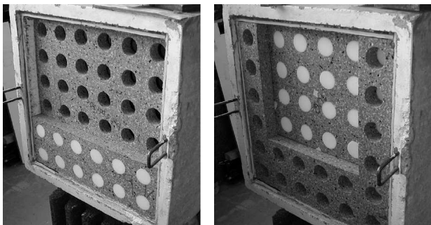
Figure 12. Preparation of the 90 mm thick heterogeneous (u160 - melamine) hybrid sample in the Big Kundt Tube. The material covers all the cross section (it is just for convenience and to better show the principle that the material does not cover all the cross section on the photography). Left: double porosity - heterogeneous, right: heterogeneous - double porosity.
