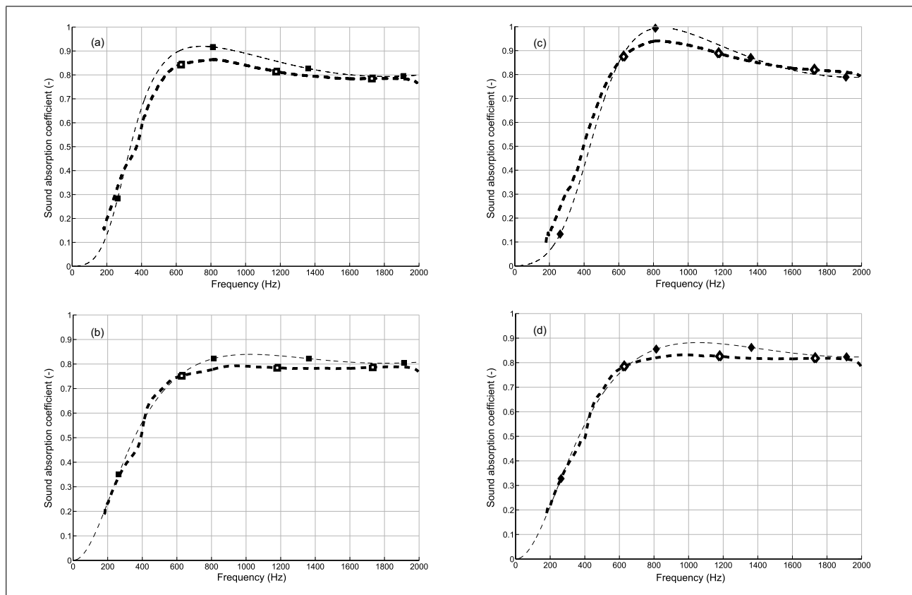
Figure 20. Medium Kundt Tube, 45.5 mm thick layer, validation for configurations A and B. (a) Configuration A, double porosity: comparison between experimental data (thick black square) and analytical model in case of F_d = 1 (thin black filled square). (b) Configuration A, heterogeneous material: comparison between experimental data (thick black square) and analytical model in case of F_d = 1 (thin black filled square). (c) Configuration B, double porosity: comparison between experimental data (thick black diamond) and analytical model in case of F_d = 1 (thin black filled diamond). (d) Configuration B, heterogeneous material: comparison between experimental data (thick black diamond) and analytical model in case of F_d = 1 (thin black filled diamond).
