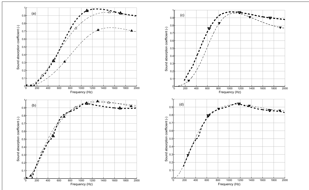
Figure 21. Medium Kundt Tube, 45.5 mm thick layer, validation for configurations C and D. (a) Configuration C, double porosity: comparison between experimental data (thick black triangle) and analytical model in case of F_d = F_d(\omega) (thin black triangle) and F_d = 1 (thin black filled triangle). (b) Configuration C, heterogeneous material: comparison between experimental data (thick black triangle) and analytical model in case of F_d = F_d(\omega) (thin black triangle) and F_d = 1 (thin black filled triangle). (c) Configuration D, double porosity: comparison between experimental data (thick black inverted triangle) and analytical model in case of F_d = F_d(\omega) (thin black filled inverted triangle) from which f_d = 1044 Hz. (d) Configuration D, heterogeneous material: comparison between experimental data (thick black inverted triangle) and analytical model in case of F_d = F_d(\omega) (thin black filled inverted triangle) from which f_d = 1044 Hz.
