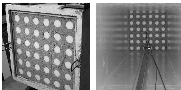
Figure 11. 90 mm thick heterogeneous (u160 - melamine) sample in the Big Kundt Tube. Left: exterior view, right: interior view.
