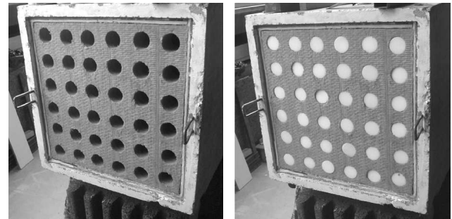
Figure 14. 90 mm thick 6 \times 6 periodical cells rockwool sample in the Big Kundt Tube. Left: double porosity, right: heterogeneous (with inclusions of melamine).
