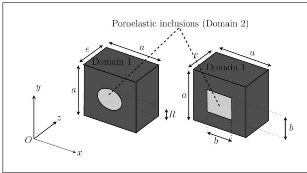
Figure 2. Considered periodic cells: circular or square cross-section for the poroelastic inclusion.
