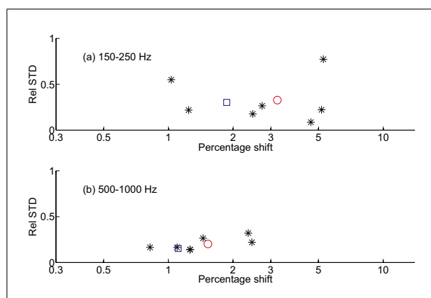
Figure 5. Results in the format of Figure 4 from 3AFC studies for shifting all mode frequencies of the datum guitar lying in (a) the band 150–250 Hz; and (b) the band 500–1000 Hz, using as input a single note (open A string). The percentage shifts corresponding to the best-four averages are (a) 1.87; (b) 1.53.
