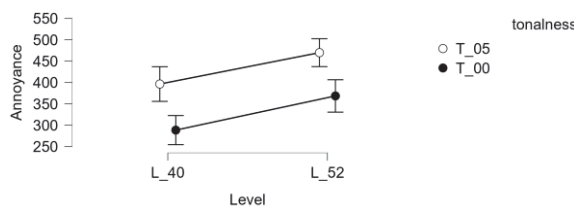
Figure 2 Influence of noise level and tonality on annoyance.
