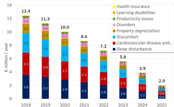
Figure 3 Social noise costs avoided (by type of effect) due to the presence of the new pavement on the A6 motorway at L'Haj-les-Roses, according to its progressive loss of acoustic effectiveness over time.
