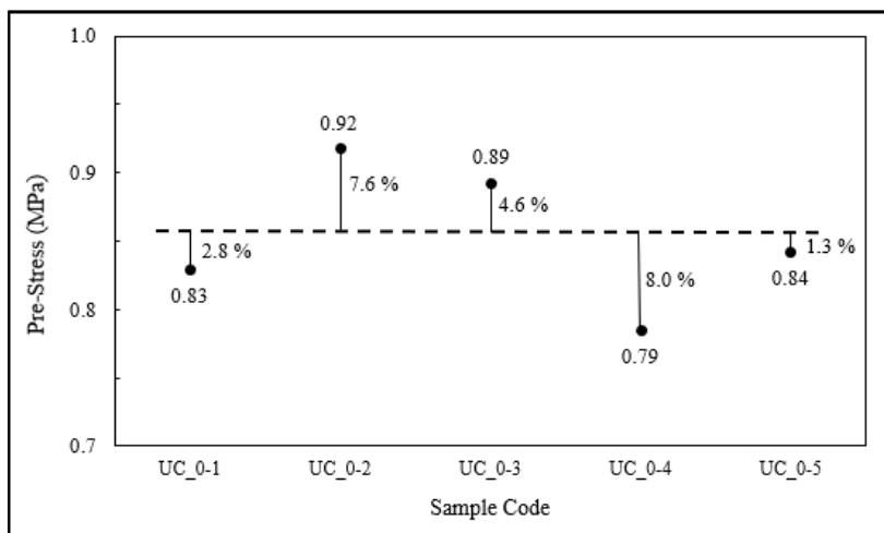
Figure 4. Calculated pre-stress values of UC_0 samples.
