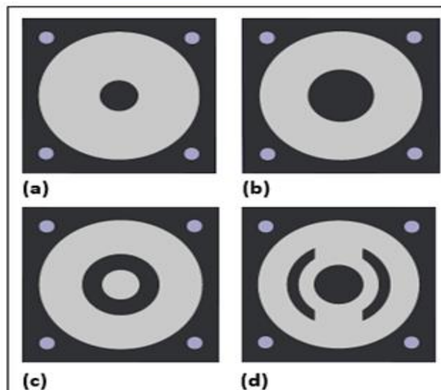
Figure 2. Unit cells: (a) UC_1 with 7 mm diameter mass; (b) UC_2 with 12 mm diameter mass; (c) UC_3 with 14 mm inner mm and 7 mm outer diameters mass; (d) UC_4 with a central mass and two identically divided arc masses.
