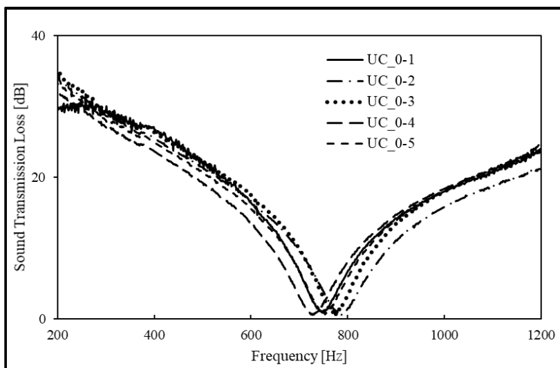
Figure 3. The curves of UC_0 samples under the bandlimited white noise excitation.
