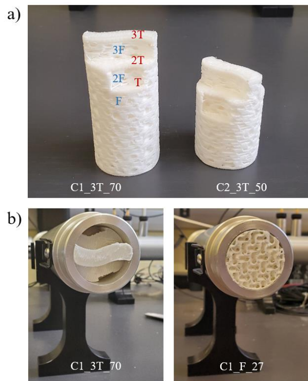
Figure 1. a) Tested samples C1 and C2, and b) impedance tube sample C1_3T_70 and C1_F_27 positioning.
