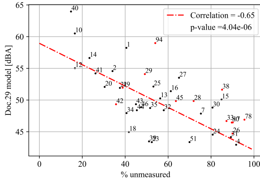
Figure 2. Percentage of undetected flights per NMT in comparison to the modelled L_{DEN} .
