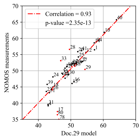
Figure 9. Measured and modelled L_{DEN} of all NMTs for the year 2023.
