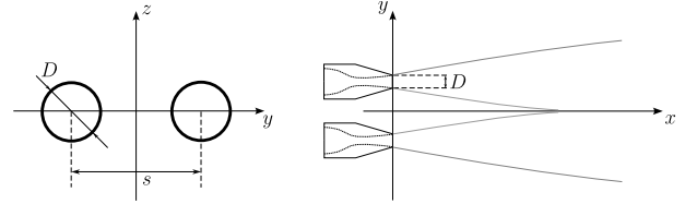
Figure 1. Sketch of the studied twin-jet configuration.
