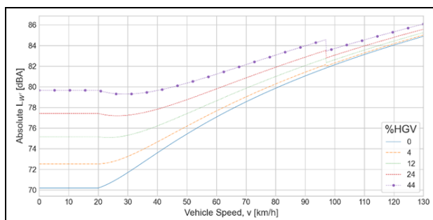
Figure 1. Vehicle speed sensitivity sweeps with composite flows: %HGV, showing discontinuity at 97 km/h.
