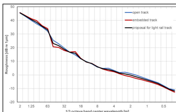
Figure 10. Proposed roughness spectrum for light rail track.
