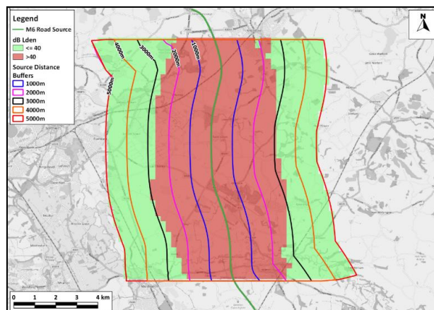
Figure 13. Propagation Distance Test – L_{den} Results.
