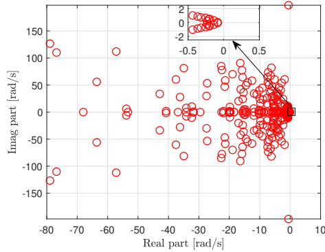
Figure 7. Eigenvalues of the ROM.
